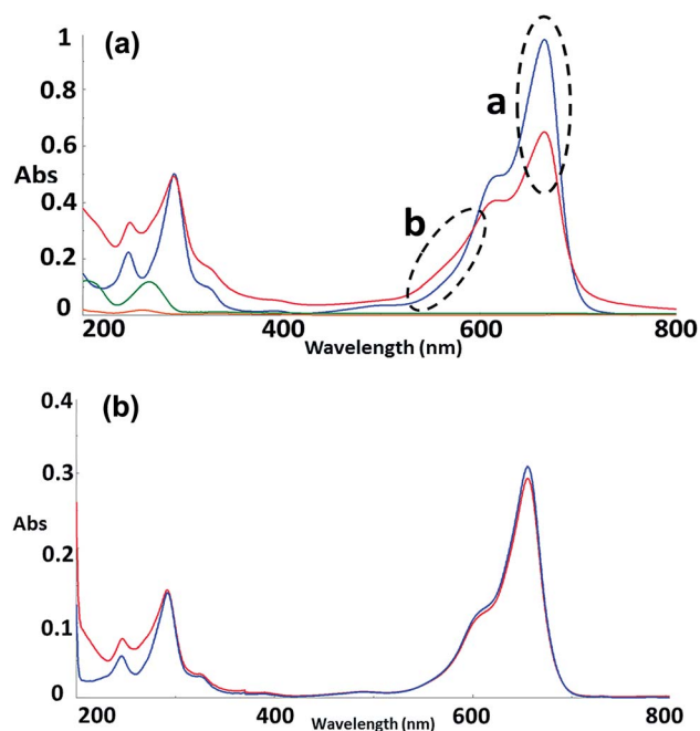
Fig. 4 (a) UV-Visible spectra in water of MB (blue), diC16dT (green), DOTAU (orange) and MB-NPs (red). “a” and “b” spectra variations. \lambda_{\text{max}} = 665 nm. (b) UV-Visible spectra of MB solution (blue) and MB-NPs (red) solution after sonication in EtOH. \lambda_{\text{max}} = 665 nm.
