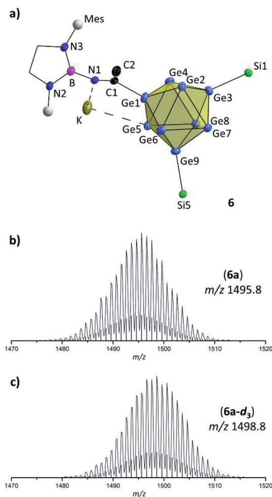
Fig. 4 (a) Molecular structure of compound 6 with -(\text{CH}_3)_2\text{CN}- moiety. All ellipsoids are shown at a 50% probability level. For clarity protons, co-crystallized solvent molecules and TMS groups are omitted. Mes fragments are indicated by grey spheres, and carbon atoms of the DAB moiety are presented as black wire sticks; (b) and (c) selected areas of ESI MS spectra (MeCN, negative-ion mode, 3500 V, 300 °C) of 6a and 6a-d 3 ; (b) molecule peak of [\text{Ge}_9\{\text{Si}(\text{TMS})_3\}_2\text{CH}_3\text{C}\equiv\text{N-DAB}^{\text{Mes}}]^- ( 6a ) at m/z 1495.8; (c) molecule peak of [\text{Ge}_9\{\text{Si}(\text{TMS})_3\}_2\text{CD}_3\text{C}\equiv\text{N-DAB}^{\text{Mes}}]^- ( 6a-d 3 ) at m/z 1498.8. Calculated isotope patterns are shown as black bars. Overview spectra are given in the ESI.†
