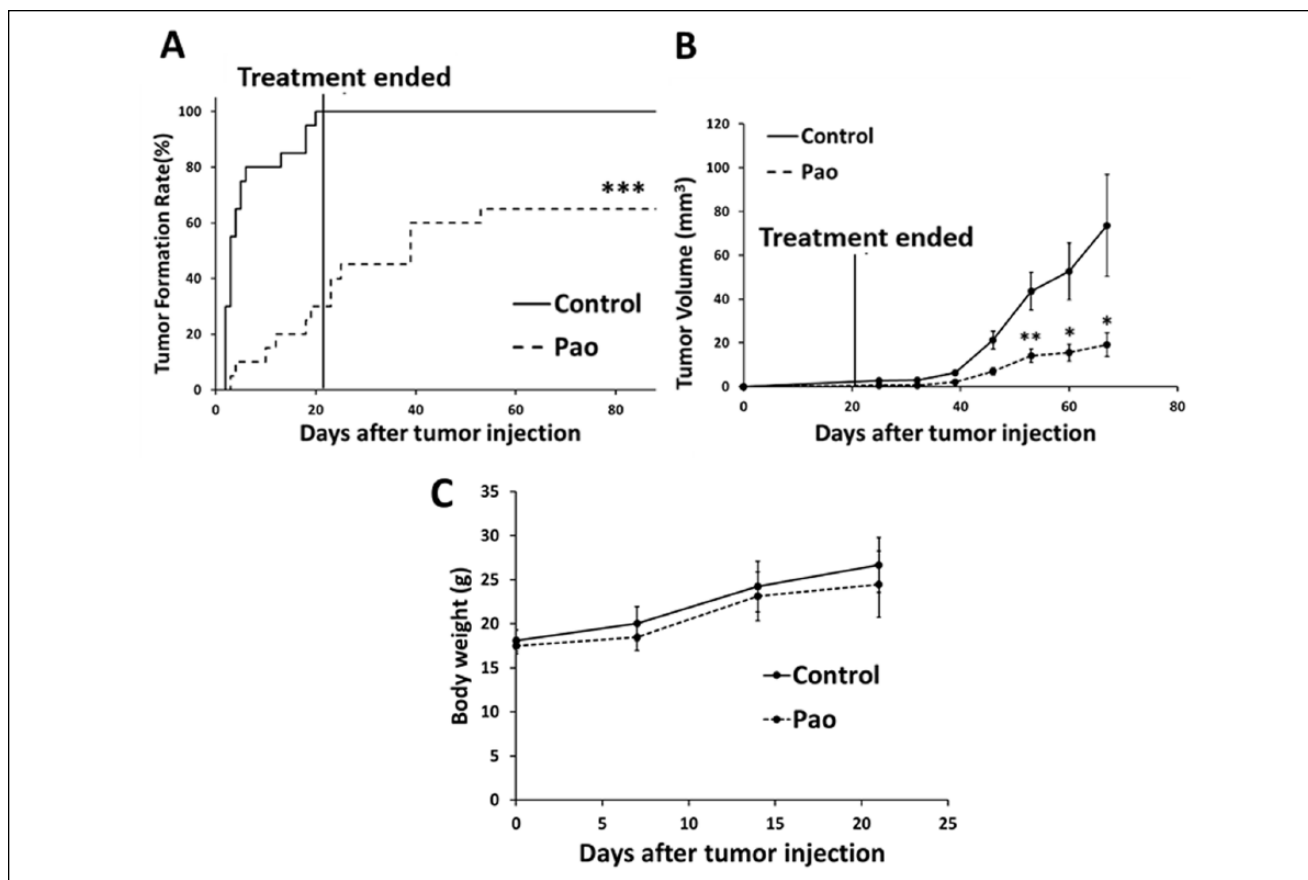
Figure 6. Effects of repeated Pao treatment on PANC-1 tumor formation and tumor growth in nude mice. (A) Tumor formation rate. A total of 2 \times 10^5 PANC-1 cells were mixed with 200 \mu\text{g}/\text{mL} Pao (Pao) or phosphate buffered saline (PBS; control), and inoculated at both flanks of nude mice ( N = 10 for each group). Treatment started the next day and lasted for 3 weeks with oral gavage of 20 mg/kg Pao (Pao) or saline (control) 5 times per week. ***P < .001 by log-rank test. (B) Longitudinal tumor growth. Tumor size was measured every 3 days by a caliper. Tumor volume = width \times width \times length/2. (C) Body weight of mice during treatment of 3 weeks. *P < .05 ; **P < .01 ; ***P < .001 compared with untreated control group.
