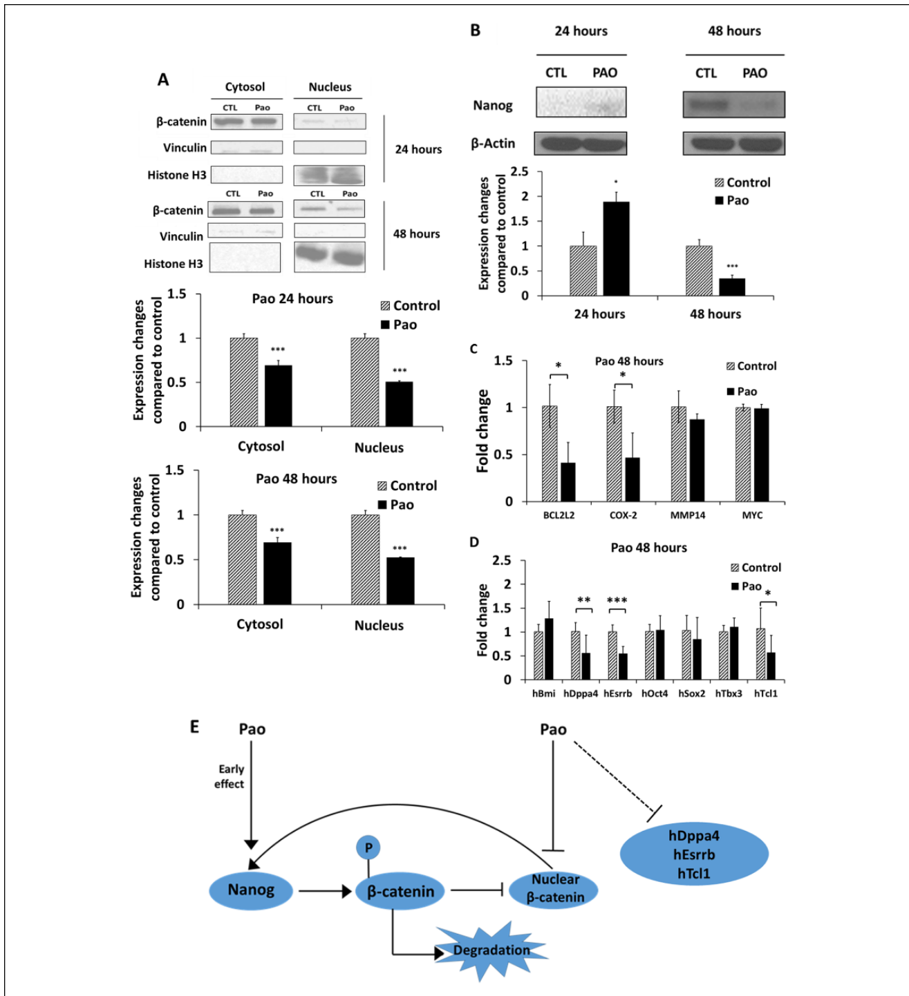
Figure 4. Decrease of gene expression related to cancer stem-like cells (CSCs) by Pao. PANC-1 cells were treated with Pao at 100 \mu\text{g}/\text{mL} for 24 and 48 hours. (A) \beta -Catenin levels in cytoplasmic and nuclear fractions, detected by Western blot. Vinculin was a loading control for cytoplasmic proteins, and histone H3 was a loading control for nuclear fraction. Bar graph shows band density normalized to loading control and compared to untreated cells. (B) The expression of Nanog, detected by Western blots. Bar graph shows band density normalized to loading control and compared to untreated cells. (C) The expression of \beta -catenin downstream target genes at 48 hours of Pao treatment, detected by RT-qPCR. (D) The expression of CSC-related genes after 48 hours Pao treatment, detected by RT-qPCR. (E) Postulated mechanism of Pao inhibiting Nanog and nuclear \beta -catenin. Pao treatment has an early effect in increasing Nanog expression, which leads to \beta -catenin phosphorylation and degradation, therefore represses nuclear \beta -catenin level. The decreasing nuclear \beta -catenin level negatively influences Nanog expression. Pao treatment may also directly inhibit \beta -catenin nuclear accumulation. Both can result in an overall suppression of both Nanog and nuclear \beta -catenin levels. Pao also inhibited the RNA level of CSC-related genes, such as Dppa4, Esrrb and Tcl1. * P < .05 ; ** P < .01 ; *** P < .001 compared with the untreated control group.
