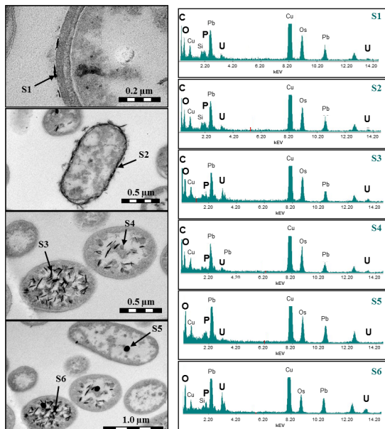
Figure 5. Transmission electron micrograph (left) of uranium precipitates deposited by the cells of Paenibacillus sp. JG-TB8 at pH 4.5 under oxic conditions. Energy-dispersive X-ray spectra (right) of the sample points (S1–S6) are marked with arrowheads. doi:10.1371/journal.pone.0102447.g005
