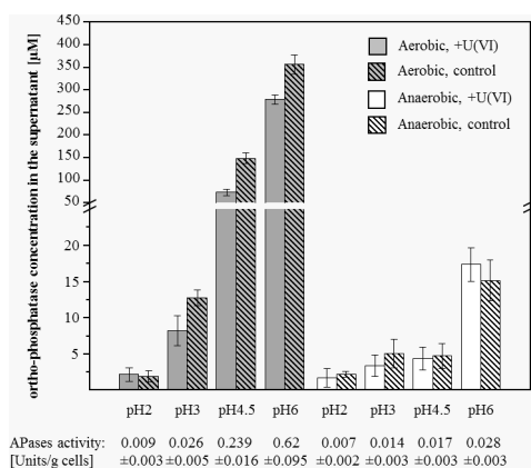
Figure 7. Amount of orthophosphate in the supernatant of cells of Paenibacillus sp. JG-TB8 after an incubation of 48 hours in dependency on pH, the aeration conditions and the presence of uranium.
