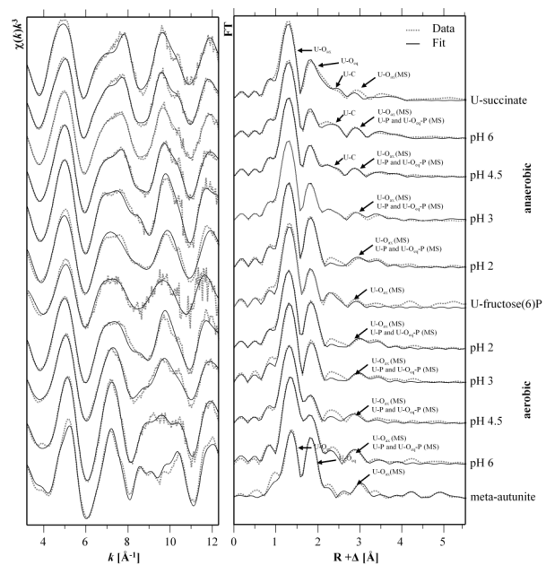
Figure 3. U L_{III} -edge k^3 -weighted EXAFS spectra (left) and the corresponding Fourier Transforms (right) ( 3.1 \text{ \AA}^{-1} < k < 12.4 \text{ \AA}^{-1} ) of the uranium complexes formed by Paenibacillus sp. JG-TB8 at pH 2, pH 3, pH 4.5, and pH 6 at different pH and aeration conditions within 48 hours. For comparison, the spectra of three model compounds, namely uranyl succinate, uranyl-fructose(6)phosphate, meta-autunite are illustrated as well. doi:10.1371/journal.pone.0102447.g003
