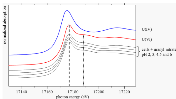
Figure 2. Uranium L_{III} -edge XANES spectra recorded from the uranium complexes formed by Paenibacillus sp. JG-TB8 at pH 2, 3, 4.5 and 6 under anoxic conditions. In addition, the XANES spectra of two solutions, which serve as reference samples for the uranium oxidation states, one of U(IV) and another one of U(VI), each at a concentration of 4 \times 10^{-2} M in 1 M HClO_4 , are shown in the figure. The dashed and the dotted line represent the position of the absorption edge of U(VI) and of the XANES peak resulting from the multiple scattering contribution of the axial oxygen atoms of U(VI), respectively. doi:10.1371/journal.pone.0102447.g002
