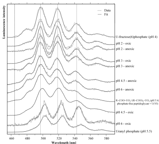
Figure 1. Normalized U(VI) luminescence spectra recorded from the uranium complexes formed under different pH and aeration conditions within 48 hours by the cells of Paenibacillus sp. JG-TB8. For comparison, dotted vertical lines indicate the main luminescence emission maxima recorded for the sample incubated at pH 2. The dashed vertical line marks the position of the luminescence emission peak which was assigned to uranyl carboxylate complexes. doi:10.1371/journal.pone.0102447.g001
