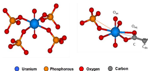
Figure 4. Structural models used for the fitting procedure of the EXAFS spectra obtained from the uranium complexes build by the cells of Paenibacillus sp. JG-TB8. The left model created from the crystall structure of meta-autunite was used for the fitting procedure of the sample incubated at pH 6 under oxic conditions. The right model contains fragments of meta-autunite (monodentate coordination at phosphate groups) as well as uranyl triacetate (bidentate coordination to carboxylic groups) and was used for the fitting procedures of all other samples. doi:10.1371/journal.pone.0102447.g004
