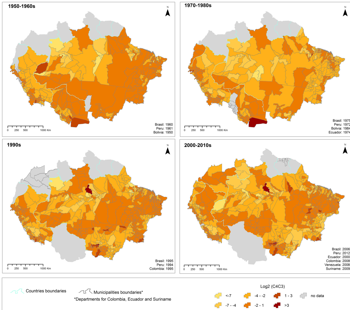
Figure 6. Ratio of C4 to C3 cropland area ( \text{Log}_2(\text{C4C3R}) ) in each municipality across groups of decades. Specific census dates grouped for each map are indicated for each period.
