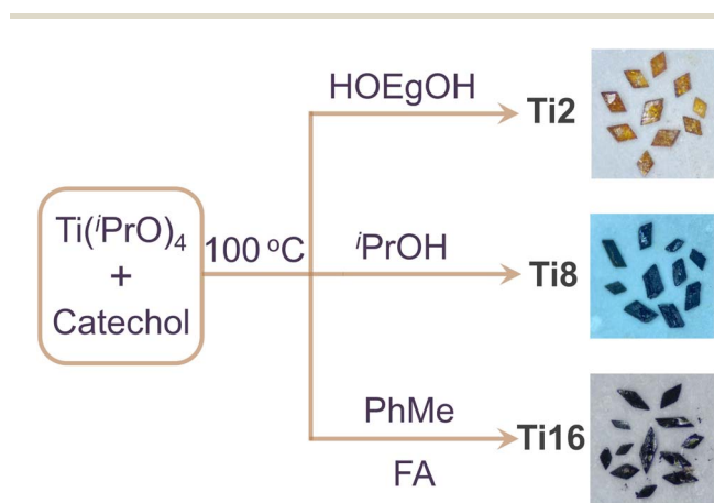
Scheme 1 Schematic diagram of the synthesis for Ti2 , Ti8 , and Ti16 (HOEGOH = ethylene glycol; i PrOH = isopropanol; PhMe = toluene; FA = formic acid).
