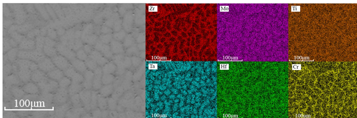
Fig. 3 Element distribution maps of HfMoTaTiZrCr 0.5 RHEA.
