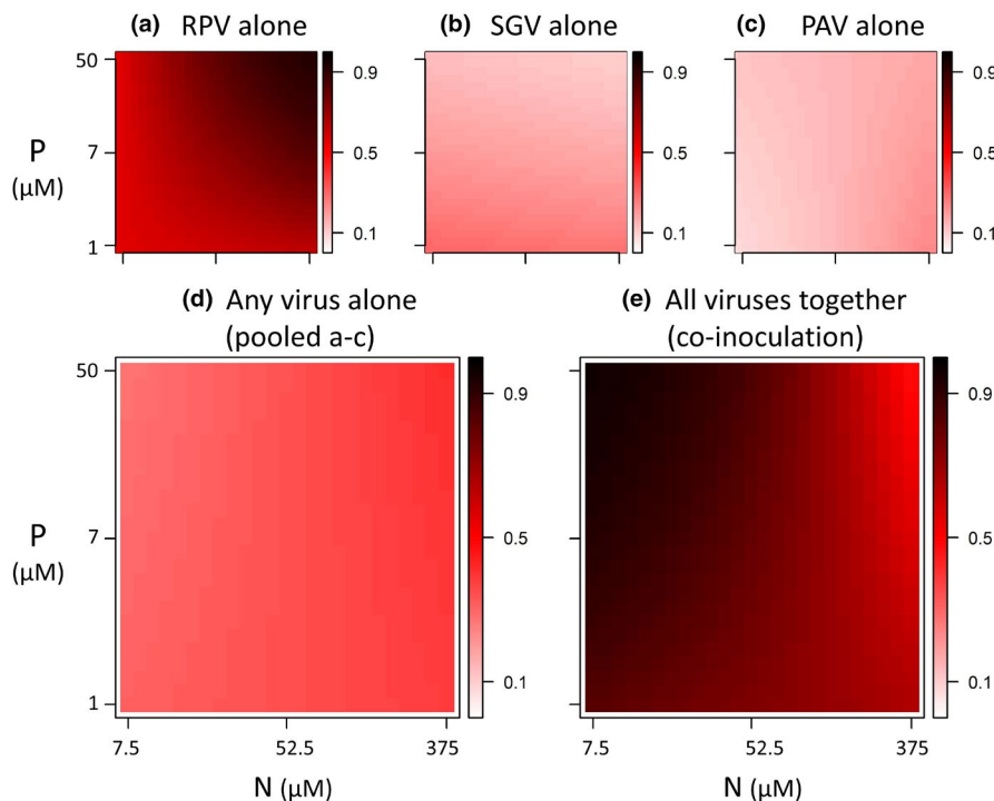
FIGURE 1 Heat maps project infection risk across gradients of nitrogen and phosphorus supply. Hosts (oats, Avena sativa ) are exposed to one or three viruses (barley/cereal yellow dwarf viruses [B/CYDV's]: CYDV-RPV, BYDV-SGV, and BYDV-PAV) along gradients of nitrogen and phosphorus supply (three levels each). Colors show impacts of resource supply on infection risk (i.e., infection prevalence; the proportion of exposed hosts that became infected), as fitted by logistic regression models. The risk of infection by each virus alone (single inoculations: A–D) qualitatively misdiagnoses the risk of infection when hosts are inoculated with all three viruses together (co-inoculations: E). (a) Risk of infection by RPV alone is higher than (b) SGV or (c) PAV, but none of the viruses respond significantly to N, P, or N:P ratio in isolation (although sample size is admittedly low—see Table S3). (d) When pooling the single inoculations (ignoring differences among viruses), infection risk for hosts does not vary with nutrients. (e) However, infection risk for hosts co-inoculated with all three viruses together is significantly higher under conditions of low N and high P (high N:P ratio). This emergent pattern arises from resource-dependent interactions among viruses within hosts (Box 1; Figure 2)
