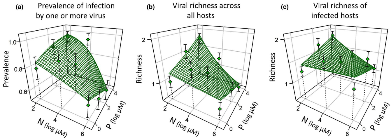
FIGURE 3 Viral richness peaks with the combination of low N and high P. Hosts (oats, Avena sativa ) are grown under combinations of nitrogen and phosphorus supply (three levels each) and co-inoculated with three viruses (barley/cereal yellow dwarf viruses [B/CYDV's]: CYDV-RPV, BYDV-SGV, and BYDV-PAV). (a) Overall prevalence among co-inoculated hosts (i.e., proportion of exposed hosts that became infected by one or more viruses) increases with the combination of low N and high P (also shown as a heat map in Figure 1e). (b) Viral richness among all co-inoculated hosts (average number of virus species per host) also increases with these resource conditions. (c) Among only the infected hosts, viral richness remains relatively constant across N and P. Planes show fits of linear models (statistics: Table 2). Error bars are standard errors. These responses of the virus community reflect the combination of each virus's responses in co-inoculated hosts (orange planes in Figure 2). Specific combinations of viruses (e.g., RPV +SGV) shown in the appendix (Figure S2)
