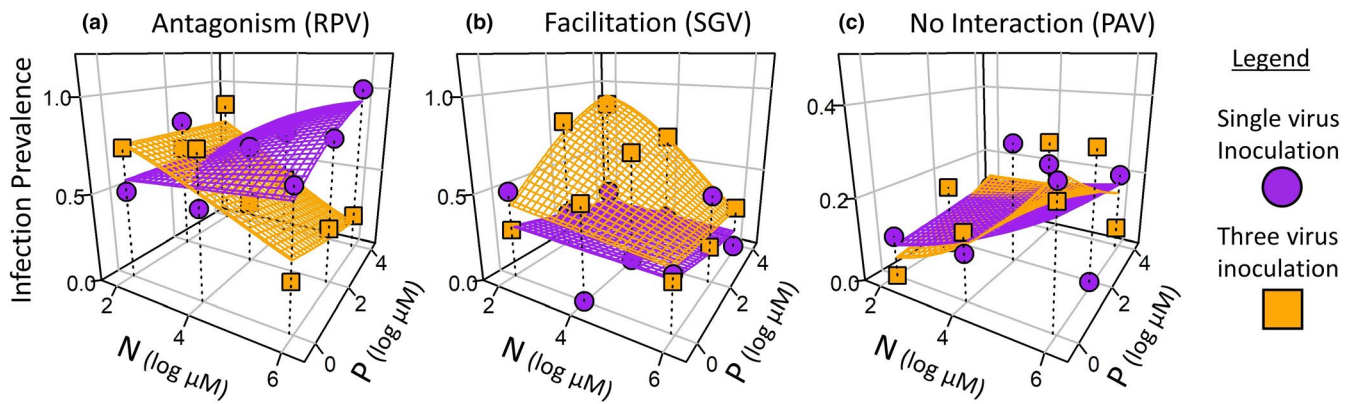
FIGURE 2 Infection prevalence of three viruses illustrates three types of resource-dependent outcomes within hosts: antagonism, facilitation, and weak or no interaction. Hosts (oats, Avena sativa ) are grown under combinations of nitrogen and phosphorus supply (three levels each) and inoculated with three viruses (barley/cereal yellow dwarf viruses [B/CYDV's]: CYDV-RPV, BYDV-SGV, and BYDV-PAV), either singly (purple circles) or jointly (orange squares). (a) Prevalence of RPV (i.e., proportion of the exposed hosts that became infected) suggests resource-dependent antagonism (e.g., competition) within hosts. Prevalence of RPV is relatively unresponsive to nutrients when alone (if anything, increasing with N) but decreases steeply with N in co-inoculations. (b) In contrast, SGV suggests facilitation. Prevalence of SGV is relatively unresponsive to nutrients when alone (if anything, decreasing with P) but increases with high P and low N in co-inoculations. (c) Finally, prevalence of PAV does not differ between single or co-inoculations and suggests weak or no interactions within hosts. Colored planes show fits of logistic regressions (statistics: Tables 1 & Table S3). Planes for single inoculations (purple) correspond to the heat maps for each virus alone (a–c in Figure 1), also shown in two dimensions (Figure S1 & Figure S3)
