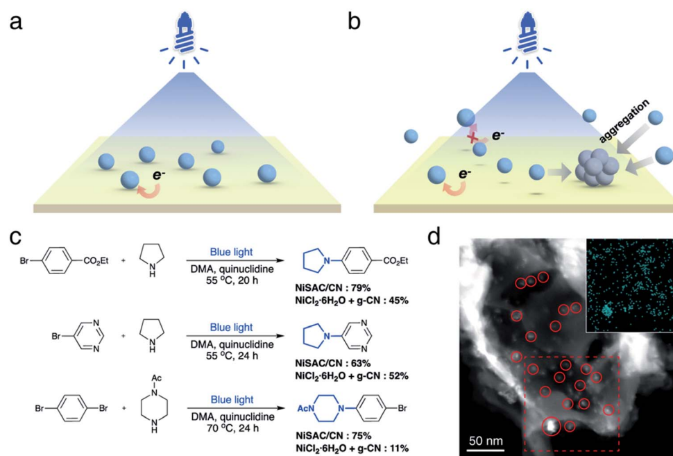
Fig. 2 The schematic picture of (a) NiSAC/CN and (b) semi-heterogeneous \text{NiCl}_2 \cdot 6\text{H}_2\text{O} and carbon nitride (blue, gray balls, and yellow sheets represent Ni atoms, Ni aggregates, and carbon nitride). (c) Comparison of yields under NiSAC/CN or semi-heterogeneous \text{NiCl}_2 \cdot 6\text{H}_2\text{O} and carbon nitride. (d) TEM image of carbon nitride after reaction under semi-heterogeneous system. * The indicated yields are the average of three replicate experiments.
