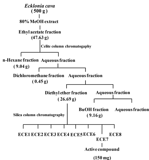
Fig. 1. Schematic of the isolation and purification of the active compound from Ecklonia cava
