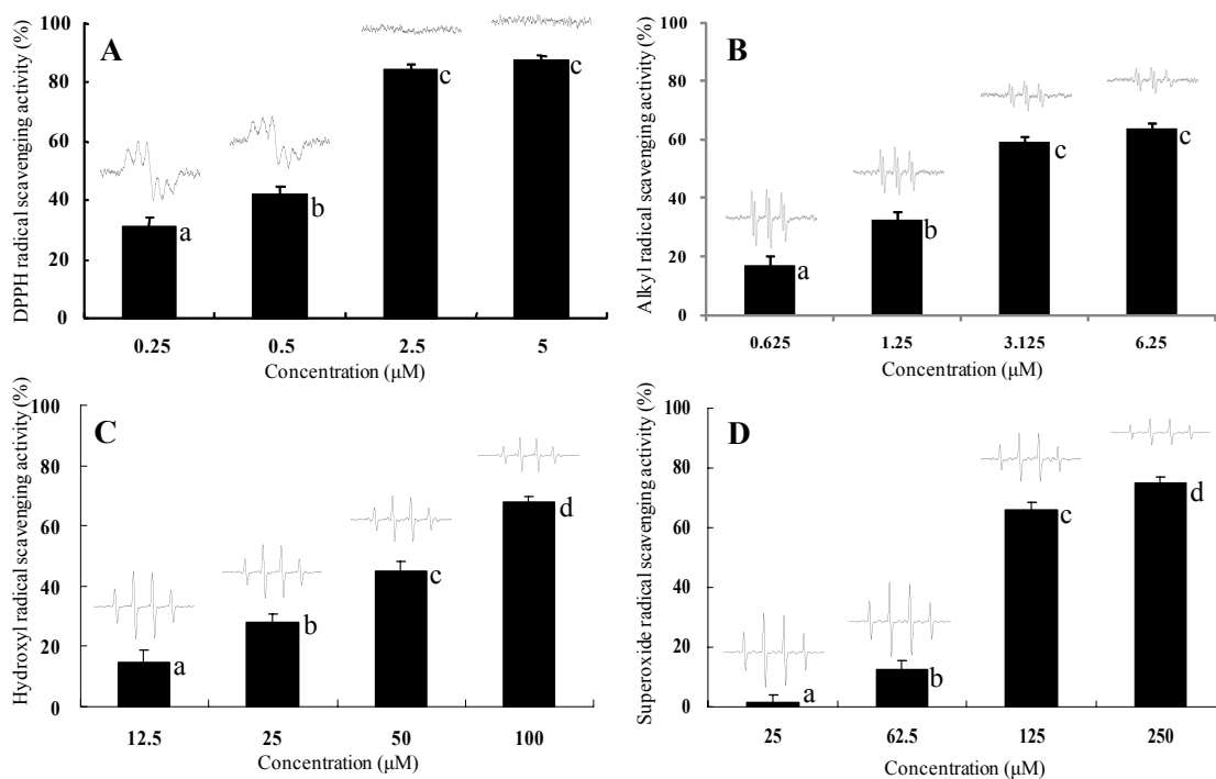
Fig. 3. Free radical scavenging activities of PPB measured using an ESR spectrometer. (A) DPPH radical; (B) Alkyl radical; (C) Hydroxyl radical; (D) Superoxide radical. Experiments were conducted in triplicate and the data were expressed as the means \pm SE. Values with different alphabets are significantly different at P < 0.05 as analyzed by Duncan's multiple range test (DMRT).
