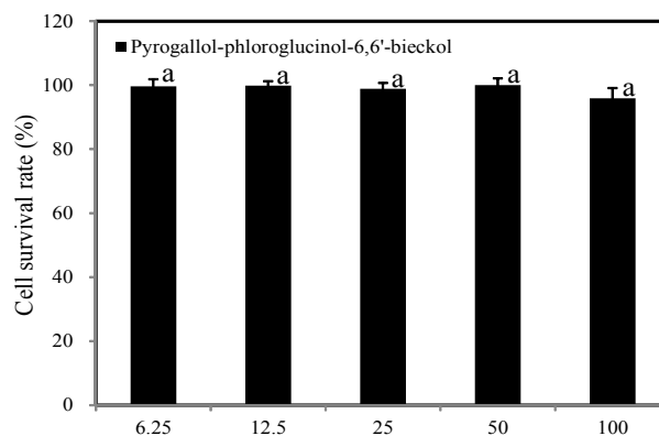
Fig. 4. The cytotoxic effect of the PPB isolated from E. cava at different concentrations. The viability of Vero cells was determined using the MTT assay. Experiments were conducted in triplicate and the data are expressed as the means \pm SE. Values with different alphabets are significantly different at P < 0.05 as analyzed by Duncan's multiple range test (DMRT).
