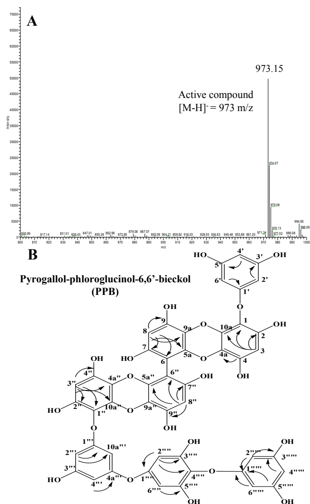
Fig. 2. MS spectroscopic and chemical structure of the active compound isolated from E. cava . The spectra were generated in negative ionization mode (A). Chemical structure and HMBC correlation of the active compound isolated from E. cava (B).
