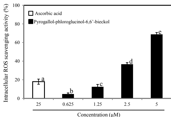
Fig. 5. Effect of the PPB on scavenging intracellular reactive oxygen species. The intracellular reactive oxygen species generated were detected via the DCFH-DA method. Experiments were conducted in triplicate and the data were expressed as the means \pm SE. Values with different alphabets are significantly different at P < 0.05 as analyzed by Duncan's multiple range test (DMRT).
