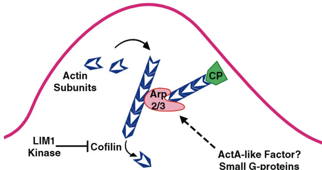
Figure 11. Model for signal-induced actin assembly at motile spots and at the leading edge. When Arp2/3 complex is activated, free barbed ends are created near the membrane, which assemble actin (blue). The mechanism for the local activation or recruitment of Arp2/3 complex at sites of assembly is unknown. Small G proteins, phosphoinositides, and an endogenous ActA-like factor may participate in the recruitment or activation of Arp2/3 complex at the membrane. Actin polymerization then proceeds at the new free barbed ends until blocked by CP. The short-lived actin filaments would subsequently disassemble via the action of cofilin. LIM-kinase-1, which inactivates cofilin and is also stimulated by GTP-rac, may regulate the disassembly of actin filaments. Spatial regulation of the processes of actin assembly and disassembly could result in the growth of filaments in the extending lamella and their subsequent disassembly at sites further from the leading edge.
