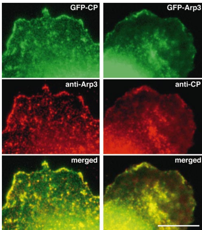
Figure 2. Arp2/3 complex and CP colocalize in punctate structures in the lamella and along the edge of cells. PtK1 cells expressing GFP-CP ( left ) or GFP-Arp3 ( right ) were fixed and labeled with antibodies to localize Arp2/3 complex ( left ) or CP ( right ), respectively. Green , GFP-tagged proteins; red , antibody labeling. Bottom , merged image of each red-green pair; yellow , regions of overlap of Arp2/3 complex and CP. Bar, 10 \mu\text{m} .
