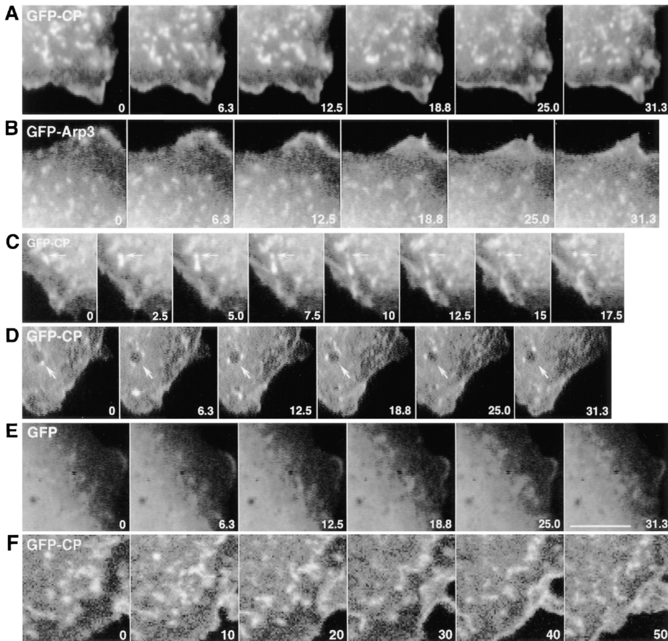
Figure 1. The distributions of GFP-CP (A, C, D, and F) and GFP-Arp3 (B) in living fibroblasts change dramatically over time. Each sequence of images (A-F) shows selected frames from a video sequence demonstrating that the distributions of GFP-CP and GFP-Arp3 change with time. Movies of the complete video sequences for A-F present these data more clearly and are available at www.cooperlab.wustl.edu or from the authors. Arrows in C and D indicate the initial position of a prominent motile spot formed in the lamella (C) or associated with a macropinosome (D). The distribution of GFP (E) is diffuse, as expected. Slight changes in the distribution of GFP over time reflect changes in cell thickness that accompany cellular movements. The sequence in F was obtained using a confocal microscope and shows that the accumulation of GFP-CP at the cell periphery is not due to increased cell thickness at the edge of the cell. Numbers in the lower corner of each image indicate elapsed time in seconds. Bar, 10 \mu m.
