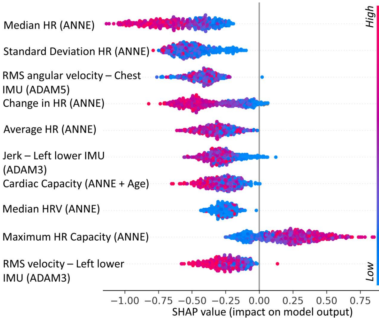
Fig. 6. Tree-based Shapley explainer for combination (Task Composite + Task Harnessing) tasks for all subjects.
