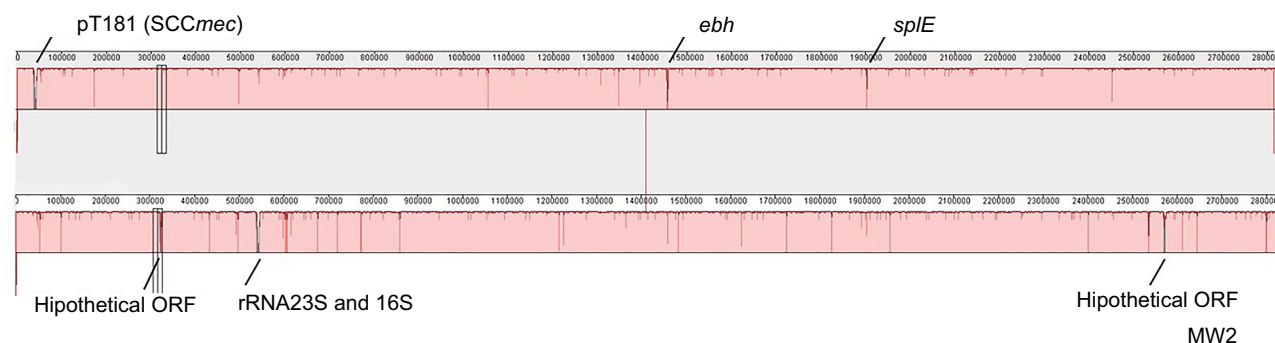
Figure S1 ProgressiveMauve alignment showing differences between 2288 and MW2 genomes.
