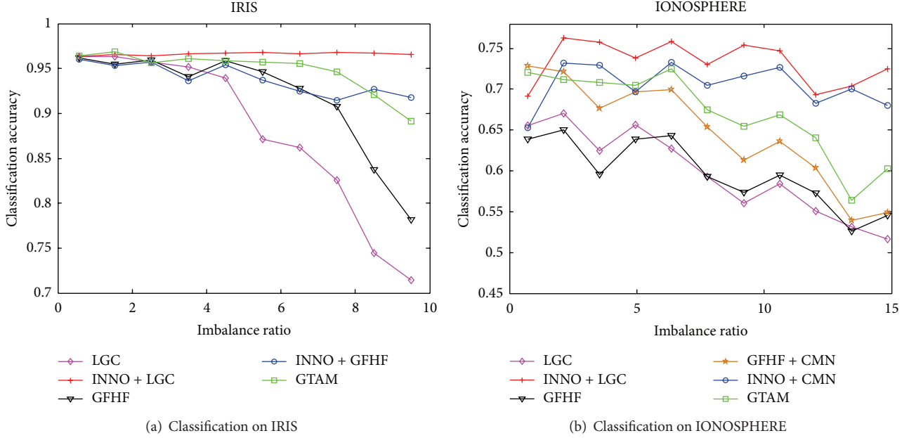
FIGURE 4: Influence of imbalanced ratio in labeled dataset to the classification accuracy.
