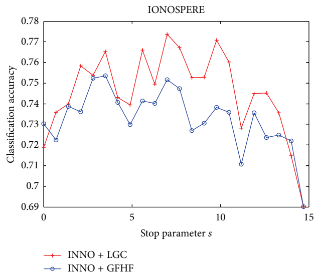
(b) IONOSPHERE
