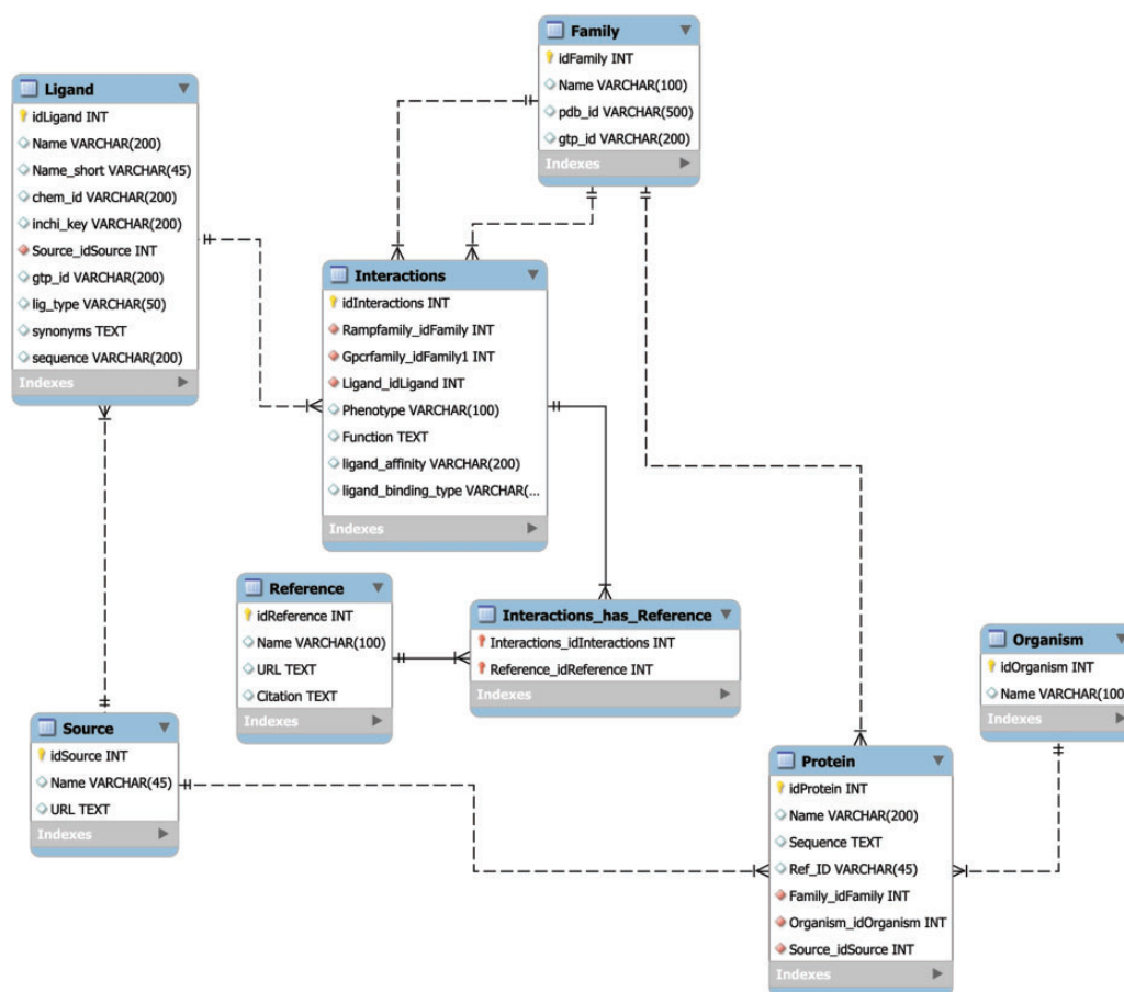
Figure 1. The RampDB data model. The MySQL database schema for RampDB, with individual tables and their connections illustrated. Primary table keys (yellow), character fields (white) and integer fields (red) are indicated. The indexes are virtual links (not shown in the schema) that are created to connect columns which are typically searched together in individual user queries.
