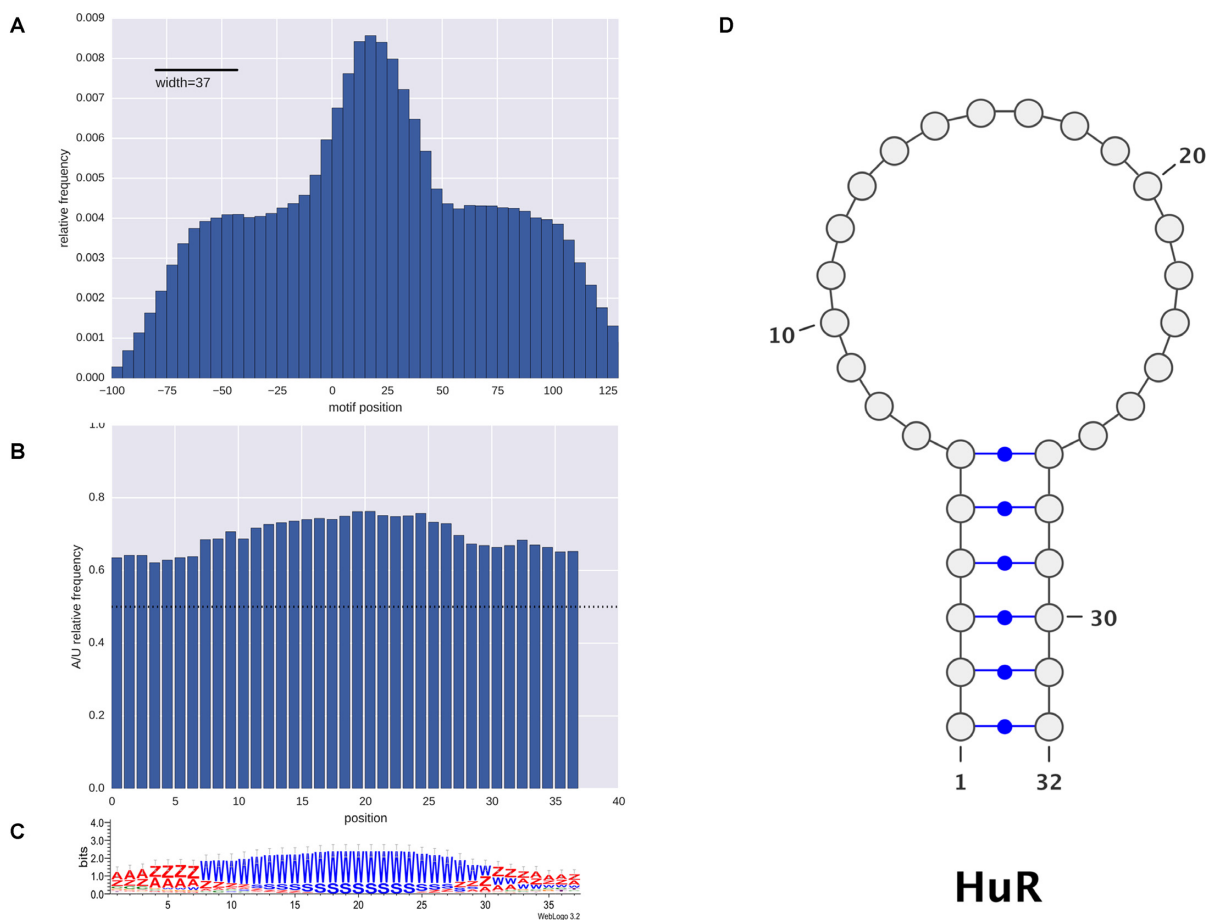
Figure 4. The HuR binding motif. (A) Histogram showing the motif position for the HuR data set. The zero of the x-axis corresponds to the start of the binding site reported in the corresponding BED file for every RNA; (B) A/U percentage of primary sequence motif corresponding to the structural motif found. The horizontal line at 50% is the value expected by chance; (C) Logo in qBEAR notation showing the structural motif; (D) Structural motif representation, showing the long loop that composes the structural signal.
