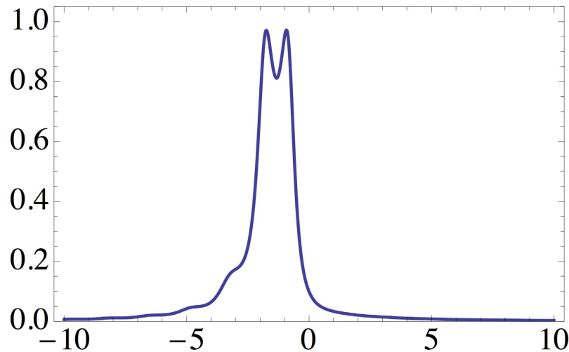
Figure 1. Transmittance T as a function of \text{Re}(n) for decay \sigma = 0.95 , c = 1.94 showing amplification of the matter wave for certain negative refraction indices n .
