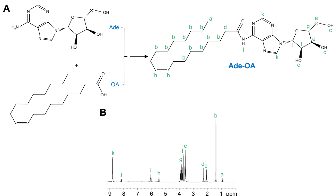
Figure 1 Synthesis scheme (A) and ^1\text{H-NMR} spectroscopy (B) of Ade-OA prodrug.
