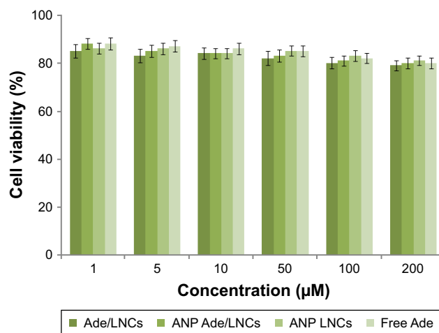
Figure 6 H9c2 cells cytotoxicity of LNCs determined using MTT assay.
