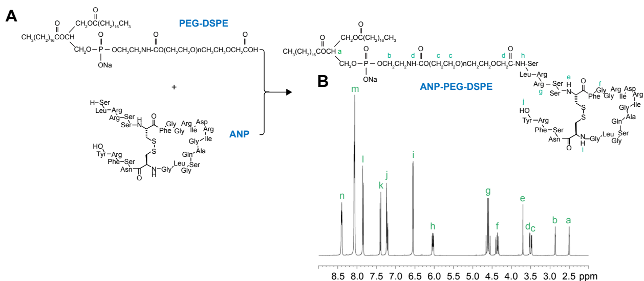
Figure 2 Synthesis scheme (A) and ^1\text{H-NMR} spectroscopy (B) of ANP-PEG-DSPE ligand.
