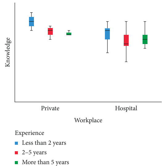
FIGURE 2: Box plot of knowledge score by health system affiliation and experience.
