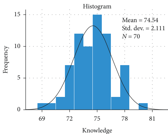
FIGURE 1: Histogram of knowledge score showing normal distribution.
