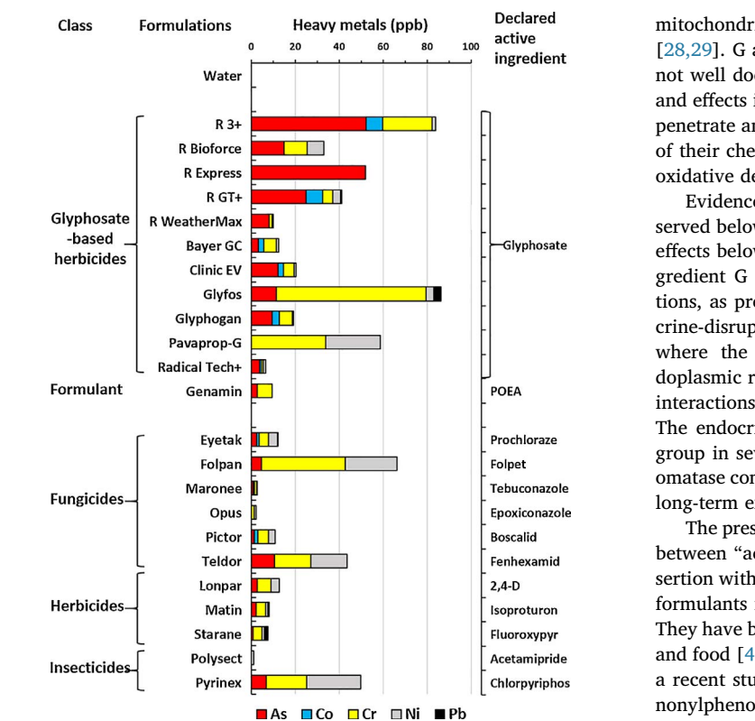
Fig. 6. Heavy metals in formulations of pesticides at their recommended dilutions.
