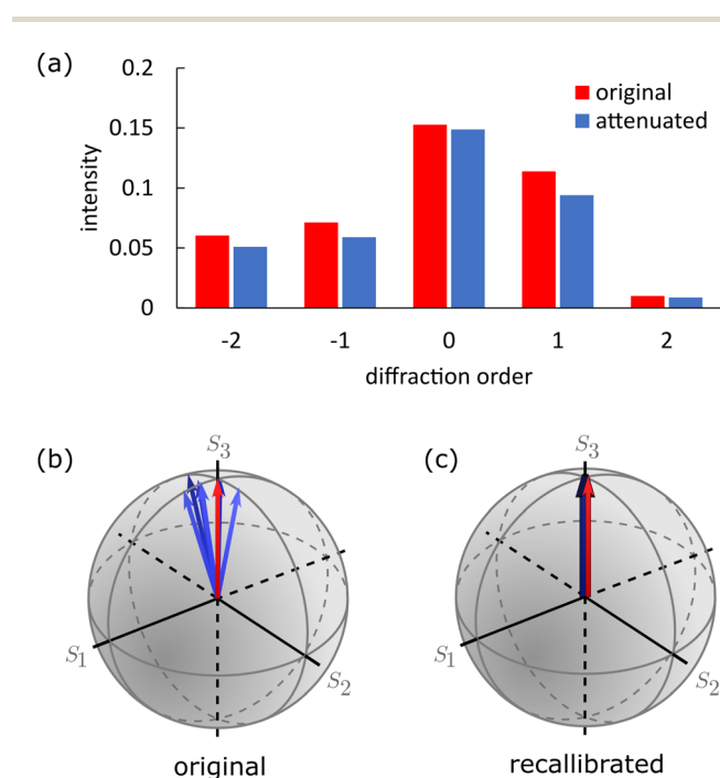
Fig. 5 (a) Measurements recorded by the camera for incident light with a polarisation of (1,0,0,1) for an imaging system working precisely as designed (red), and for a system with errors introduced (blue), where we apply nonpolarising attenuation of a random value up to 10% to each measurement independently. (b) The original incident state (red) and the reconstructions of the poisoned states using every possible combination of four or five measurements. The reconstructed vectors diverge in different directions from the incident state, indicating errors are present. (c) Recalibration of the reconstruction matrices allows us to correctly reconstruct the polarisation with the same imaging system.
