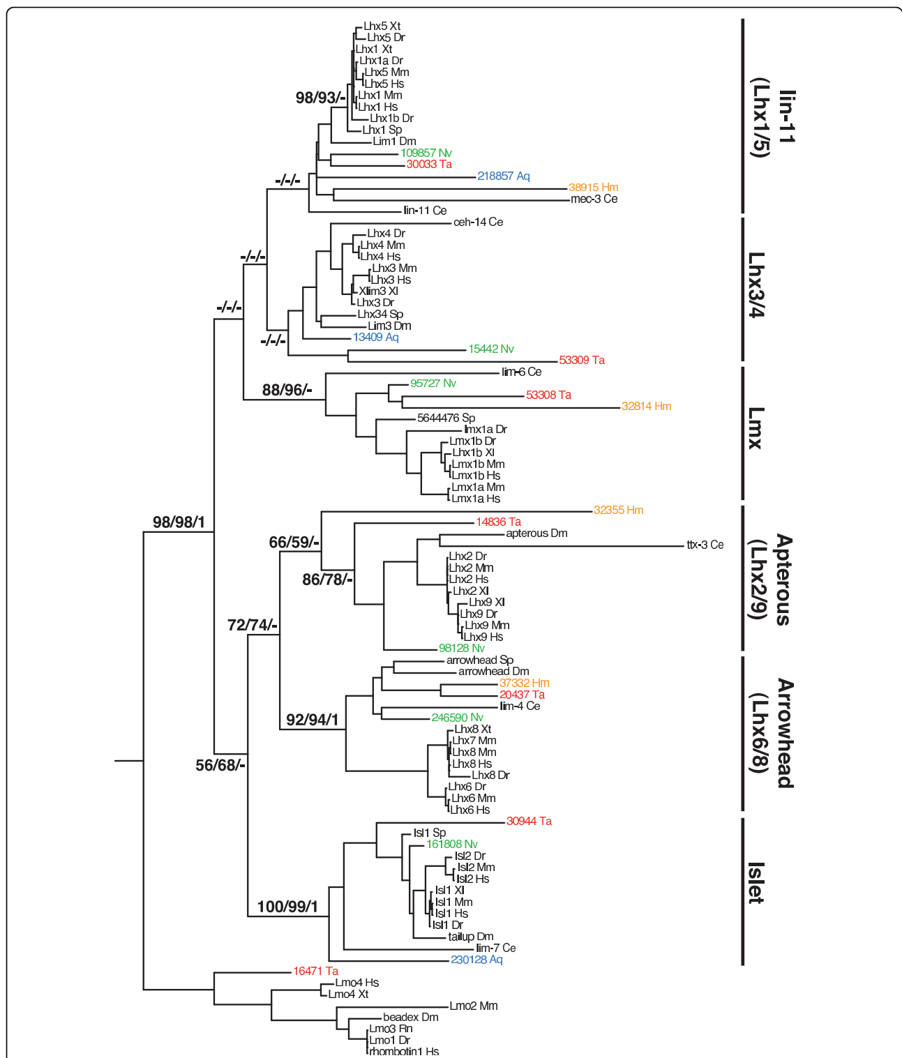
Figure 1 Phylogeny of LIM homeobox genes. The maximum likelihood tree based on an alignment of two LIM domains and the homeodomain is shown here with support values from Neighbor-joining/Likelihood/Bayesian analyses shown for the major nodes (relationships within the major classes were well supported only for vertebrate sequences). Neighbor-joining and Likelihood bootstrap values above 50% are shown, as are Bayesian posterior probabilities above 0.95. Full trees from each analysis are shown in Additional file 1. Aq = Amphimedon queenslandica (blue); Ce = Caenorhabditis elegans ; Dm = Drosophila melanogaster ; Dr = Danio rerio ; Hm = Hydra magnipapillata (orange); Hs = Homo sapiens ; Nv = Nematostella vectensis (green); Rn = Rattus norvegicus ; Sp = Strongylocentrotus purpuratus ; Ta = Trichoplax adhaerens (red); Xt = Xenopus tropicalis .
