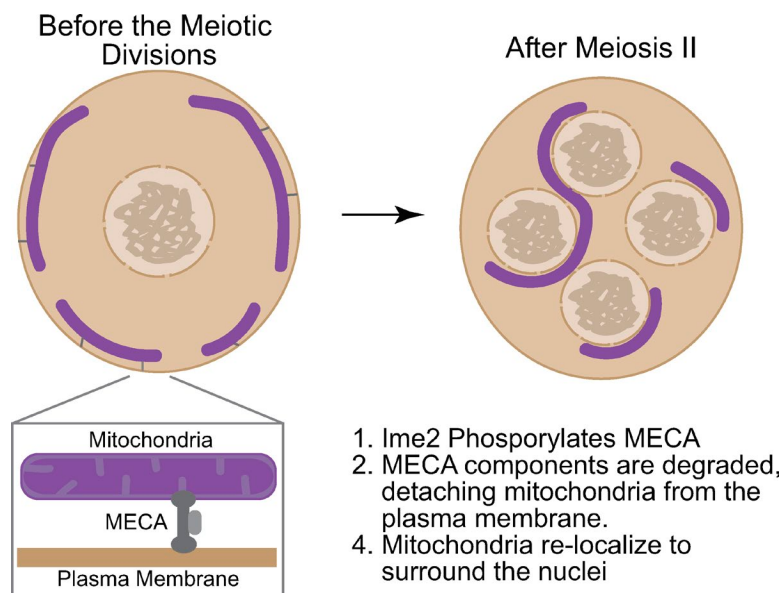
Figure 1. Mitochondrial remodeling during meiosis. Before the meiotic divisions, tubular mitochondrial networks (shown in purple) are tethered to the plasma membrane by MECA. As cells enter the meiotic divisions, IME2 expression is highly induced by the transcription factor Ndt80. In meiosis II, Ime2 phosphorylates MECA proteins Num1 and Mdm36, leading to their destruction. The mitochondria are released from the cell cortex and associate around the nuclei.
