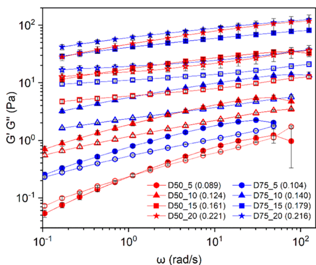
Figure 7. Storage ( G' —full symbols) and loss ( G'' —empty symbols) moduli as a function of frequency for dispersions with different particle concentrations and fixed XG concentration (red symbols: 0.50%, blue symbols: 0.75 wt %). The values in parentheses in the legend refer to the volume fraction of PLA particles in the samples. See Table 1 for the decoding of the acronyms in the legend. Error bars are calculated as standard deviation (eq 8).
