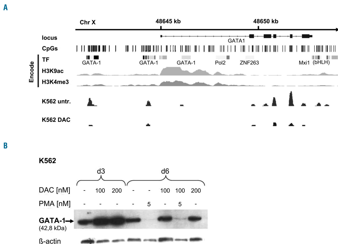
Figure 7. Decitabine induces gene demethylation and expression of the erythroid-specific transcription factor GATA1 in K562 cells. (A) Schematic representation of the GATA1 gene locus. The GATA1 gene is depicted as a black line from 5' (left) to 3' (right) with exons represented as boxes. CpG density (CpGs) is indicated by vertical bars. Transcription factor (TF) binding sites were determined through combined TF chromatin immunoprecipitation sequencing (ChIP-seq) experiments from different tissues/cell lines published by the ENCODE consortium. Likewise, activating histone marks H3K9ac and H3K4me3 are taken from ChIP-seq experiments in untreated K562 cells which were published and made publicly available from the ENCODE consortium. DNA methylation was assessed by enrichment through methyl-CpG immunoprecipitation sequencing experiments in untreated K562 cells (K562 untr.) and in K562 cells treated with decitabine (K562 DAC). (B) K562 cells were treated with three 24 h pulses of 100 nM or 200 nM decitabine and harvested on days 3 and 6. PMA 5 nM was added to the culture media for the final 48 h. Immunoblotting of whole cell lysates with rat anti-GATA1. Immunoblotting with mouse anti-beta-actin was performed to control for lane loading.
