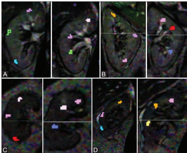
Image1: FA and ADC value in various stages of chronic kidney disease (CKD stage I >90, CKD stage II 60–90, CKD stage III 30–59, end-stage renal disease CKD stage V 15–29 ml/min/1.73m 2 ). (A) Mean FA medulla and ADC cortex values in stage I diabetic patients with eGFR-113 are 0.433 \pm 0.126 and 2.168 \pm 0.187 , respectively. (B) Mean FA medulla and ADC cortex values in stage II diabetic patients with eGFR-81 are 0.394 \pm 0.146 and 1.750 \pm 0.196 , respectively. (C) Mean FA medulla and ADC cortex values in stage III diabetic patients with eGFR-51.3 are 0.384 \pm 0.086 and 1.610 \pm 0.225 , respectively. (D) Mean FA medulla and ADC cortex values in diabetic patient in end-stage CKD V with eGFR-11.2 ml/min/1.73m 2 are 0.373 \pm 0.101 and 1.540 \pm 0.310 \times 10^3 mm 2 /s, respectively. Hence, a continuous declining trend in FA values of medulla and cortical ADC values from CKD stage I to end-stage renal disease (CKD 5) was observed. However, FA values of cortex and ADC values of medulla did not show any specific trend
