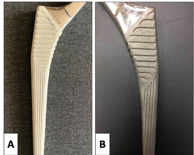
Fig. 4 Retrieved element stem. A Element Stem prior to implantation. B Element stem retrieved after revision for aseptic loosening. Demonstrated is the uniform loss of hydroxyapatite coating, likely secondary to resorption and abrasion
