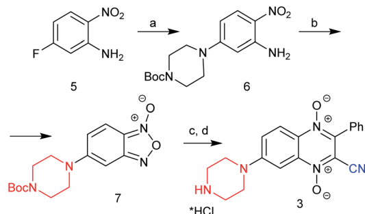
Scheme 1 New route for the synthesis of 7-(piperazin-1-yl)-quinoxaline-2-carbonitrile 1,4-dioxide ( 3 ). Reagents and conditions: (a) 1-Boc-piperazine, DMF, TEA, 50 °C, 4 h, 86%; (b) NaOCl, KOH(aq), DMF, 0–5 °C, 10–15 min, 81%; (c) BzCH 2 CN, Et 3 N, CHCl 3 , r. t., 3 h, 71%; (d) HCl/MeOH, r. t., 68%.
