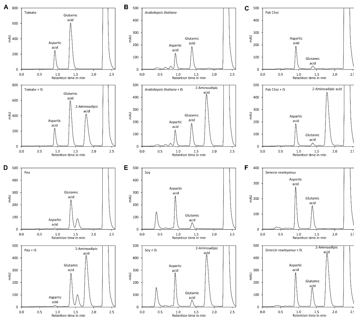
Figure 2. 2-Aminoadipic acid is not present in plant samples. (A) Chromatogram of a tomato extract (5 \mu\text{L} tomato extract were derivatised in a reaction with a total volume of 120 \mu\text{L} derivatised with DNFB and analysed by UHPLC with a flow rate of 1 mL/min. The sample in the upper panel was not spiked, the sample in the lower panel was spiked with 10 \mu\text{L} of 2-aminoadipic acid 1000 mg/L. All other samples were treated in the same way and analysed without spike (upper panels) and spiked with 10 \mu\text{L} of 2-aminoadipic acid 1000 mg/L (lower panels); (B) Sap of Arabidopsis thaliana leaves (30 \mu\text{L} ); (C) Sap of pak choi petioles (30 \mu\text{L} ); (D) Sap of unripe peas (2 \mu\text{L} ); (E) Sap of soy leaves (20 \mu\text{L} ); (F) Sap of Senecio rowleyanus leaves (30 \mu\text{L} ).
