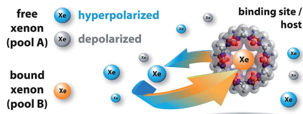
Fig. 1 Probing reversible, labile binding in a molecular cavity with xenon: free xenon atoms (pool A, where blue indicates hyperpolarized Xe and gray indicates depolarized Xe) undergo constant exchange with the binding site/host ( i.e. , cucurbit[6]uril, CB6; transparent overlay of the ball-stick-model of the molecule with its van der Waals radius representation; molecular modeling in Fig. S1 in the ESI†). The NMR signal of bound Xe shows a remarkably large chemical shift (indicated by orange xenon atoms; pool B). The host geometry with the two opposing portals facilitates fast dissociation of the complex. This causes detrimental line broadening, precluding conventional NMR detection.
