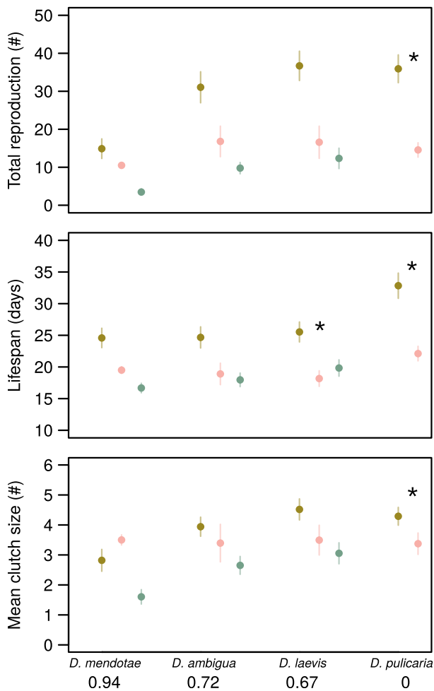
Figure 1. Significant costs of resistance (denoted with an asterisk; *), and infection (universal except for mean clutch size of D. mendotae ) with respect to three host fitness measures (mean \pm 1SE). Mean clutch size and total reproduction were quantified as the number of offspring per clutch and the total number of offspring an individual produced after infection challenge. Lifespan was scored as total lifespan of the host. Host susceptibility, defined as the fraction of hosts exposed to the pathogen that became infected, is given in parentheses next to the host species name.
