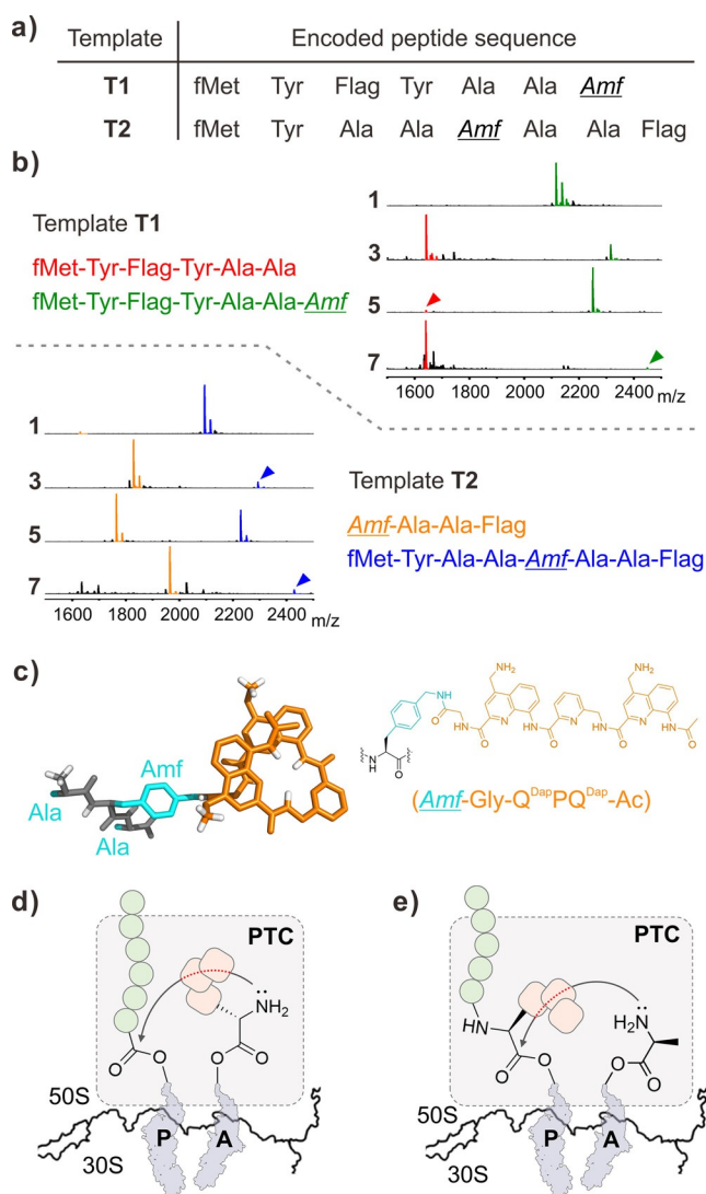
Figure 2. a) Template-encoded peptides containing Amf(-Gly-foldamer) at the C-terminus (from T1) and within the peptide (from T2). “Flag” stands for DYKDDDDK. b) Characteristic MALDI-TOF-MS spectra of resulting peptides containing 1 , 3 , 5 or 7 as a positively charged foldamer sidechain. Desired products are indicated by green and blue peaks. Side-products corresponding to unsuccessful peptidyl transferase reactions are indicated by red and orange peaks (magnification of the peaks corresponding to the desired products, along with the [M+Na]^+ and [M+K]^+ are available in the Supporting Information). c) Molecular model of Ala-Amf(-Gly-Q Dap PQ Dap -Ac)-Ala illustrating the size of the foldamer with respect to the peptide chain (left) and its extended chemical structure (right). Nonpolar hydrogen atoms have been omitted for clarity. d) Scheme of the nucleophilic addition of the foldamer-containing Amf residue on the peptidyl tRNA ester at the P-site. e) Nucleophilic addition of the Ala amine following the Amf residue. In (d) and (e) green circles and rounded squares represent elongating amino acids and aromatic residues on Amf, respectively. The red dashed part of the reaction arrow represents potential obstacles caused by the foldamer-containing residue. PTC: peptidyl transferase center.
