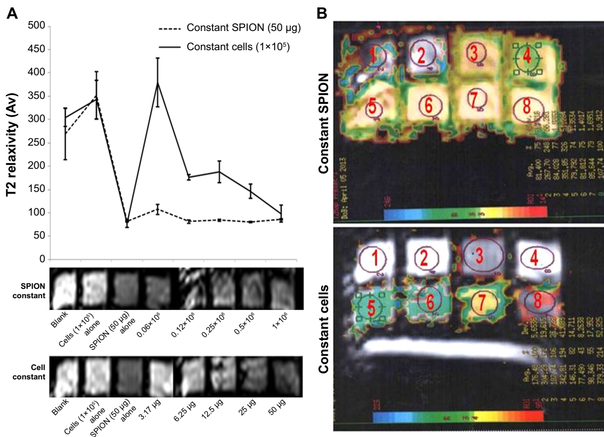
Figure 6 (A) An MRI of the phantom gel was performed to measure the T2 relaxivity of the SPION complex-labeled cells using 3TMR. Two experimental set-ups were designed, one with fixed SPION concentration (50 \mu\text{g}/\text{well} ) and variable cell numbers (0.0625– 1.0 \times 10^6 cells) and another with a fixed cell number ( 1 \times 10^5 cells) and different SPION concentrations (3.175–50 \mu\text{g}/\text{well} ). (B) Parameters for coronal T2-weighted TSE imaging used during scanning were as follows: TR, 6250 ms; TE, 150 ms; field of view, 190 \times 230 \text{ mm}^2 ; slice thickness, 2 mm; acquisition time, 5 minutes; echo train length, 16; and voxel size, 0.6 \times 0.8 \times 2 \text{ mm}^3 . SPIONs alone, unlabeled cells and gelatin alone served as MRI controls. Abbreviations: MRI, magnetic resonance imaging; 3T, 3 tesla; SPION, superparamagnetic iron oxide nanoparticle; TSE, turbo spin echo; TR, repetition time; TE, echo time.
