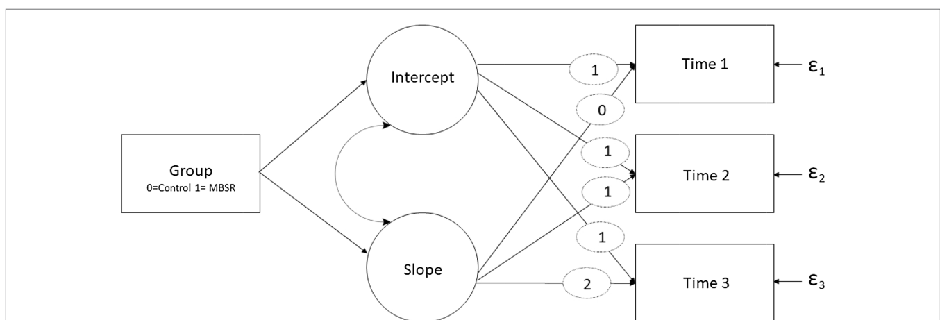
FIGURE 2 | An illustration of the individual growth curve model. The rectangles represent observed variables, while the circles represent latent factors. Curved arches represent correlations and \epsilon represents residual random parts. Fixed weights for intercept and time weight for slopes are represented by ellipses.
