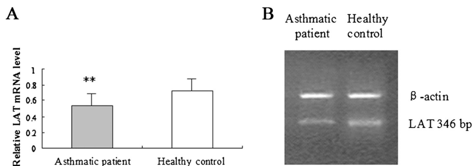
Figure 1 Expression of LAT mRNA in peripheral blood T cells in asthmatic patients and healthy controls. A) The mRNA expression of LAT was determined by real-time PCR in peripheral blood T cells from asthmatic patients and healthy controls, which was normalized to \beta -actin. The ratio of LAT/ \beta -actin was determined as the relative content of LAT mRNA. Data is shown as mean \pm SD, n = 10 (* p < 0.05 ). B) Image of RT-PCR analysis of LAT expression in asthmatic patients and healthy controls.
