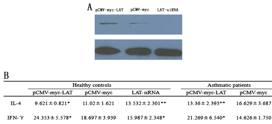
Figure 2 Overexpression of LAT inhibits Th2 cytokine production and promoted Th1 cytokine production in human peripheral blood T cells in both asthmatic patients and healthy controls. Purified peripheral blood T cells from allergic asthmatic patients and healthy controls were nucleofected with pCMV-myc-LAT, pCMV-myc, LAT-siRNA plasmids separately. A) LAT expression was analyzed by western blot. B) Nucleofected T cells were activated with anti-CD3 and anti-CD28 for 24 h. Cytokine production of IL-4 and IFN- \gamma was measured by ELISA. Data is shown as mean \pm SD, n = 10 (*p < 0.05).
