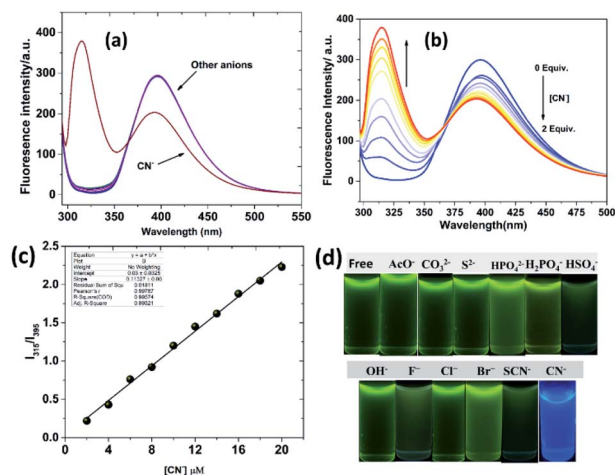
Fig. 2 (a) Fluorescence spectra of dye BBCN ( 10 \mu\text{M} ) in the presence of various anions in the solvent medium of \text{CH}_3\text{CN}/\text{HEPES} in water (7 : 3 v/v) at pH 7.2. (b) Fluorescence spectra of BBCN ( 10 \mu\text{M} ) upon the incremental addition of \text{CN}^- in \text{CH}_3\text{CN}/\text{HEPES} in water (7 : 3 v/v) at pH 7.2. \text{CN}^- concentrations were varied from 0 to 20 \mu\text{M} . (c) The linear relation of I_{315}/I_{395} for the concentration of \text{CN}^- in the range of 0– 20 \mu\text{M} . (d) Fluorescence colour change of BBCN over the addition of various anions when viewed under the UV lamp.
