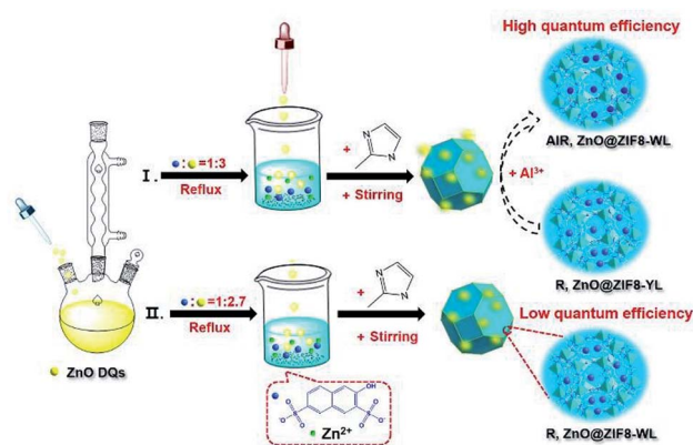
Fig. 1 Schematic of the synthesis process for the white light R,ZnO@ZIF8-WL, yellow light R,ZnO@ZIF8-YL, and in situ aluminium ions regulation for AIR,ZnO@ZIF8-WL.
