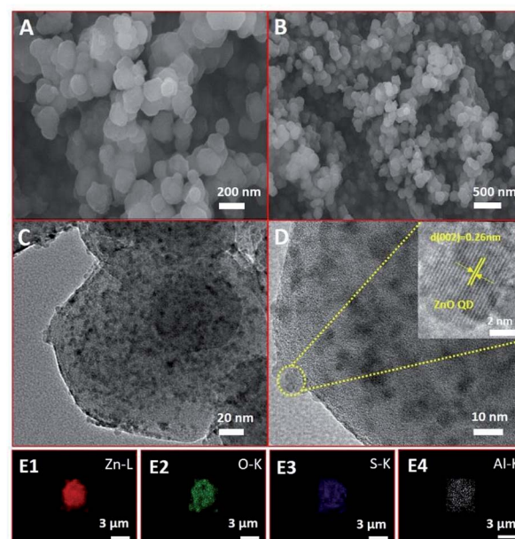
Fig. 2 (A) and (B) SEM images of AIR,ZnO@ZIF8-WL. (C) and (D) TEM images of AIR,ZnO@ZIF8-WL (the inset of (D) shows a HRTEM image of a ZnO QD, revealing a lattice spacing of 0.26 nm that arises from the (002) plane of the ZnO QD). (E1)–(E4) Elemental mapping of AIR,ZnO@ZIF8-WL.
