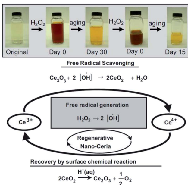
Fig. 6 Top: Observation of change in color when, cerium oxide nanoparticle coated with dextran was treated with H_2O_2 at different time intervals. Bottom: Schema of chemical reaction showing auto-regenerative properties cerium oxide nanoparticles and possible mode of mechanism data of the cerium oxide nanoparticle autocatalytic behavior and free-radical scavenging property (reproduced from M. Das et al. , Biomaterials , Elsevier, 2007 (ref. 105)).
