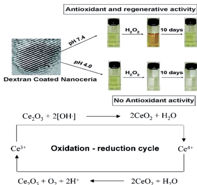
Fig. 7 Top: Color change in solutions of cerium oxide nanoparticle coated with dextran at basic and acidic pH environment on addition of H_2O_2 . Bottom: Detailed probable revised mode of mechanism data cerium oxide nanoparticle auto-regenerative attribute and free-radical scavenging property (reproduced from J. M. Perez et al. , Small , John Wiley and Sons, 2008 (ref. 106)).
