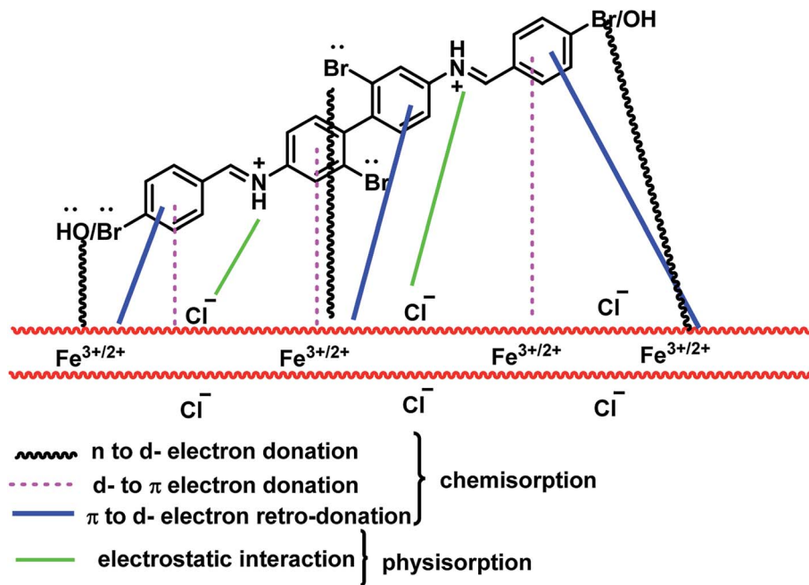
Fig. 8 Proposed model of adsorption of the synthesized Schiff base inhibitors on mild steel in 0.5 M HCl.
