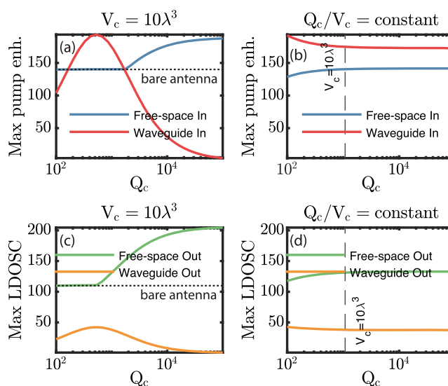
Figure 5. Maximum achievable pump enhancement (a, b) and LDOSC (c, d) as a function of the cavity quality factor Q_c for both input and output configurations; (a) and (c) are given for a fixed-mode volume V_c = 10\lambda^3 , whereas (b) and (d) are given for a constant-cavity Purcell factor Q_c/V_c . The antenna frequency is \omega_a/(2\pi) = 460 THz, and the cavity frequency is fixed at \omega_c = \omega_a - \Omega_m . The horizontal dotted line corresponds to the free-space case with only the bare antenna.
