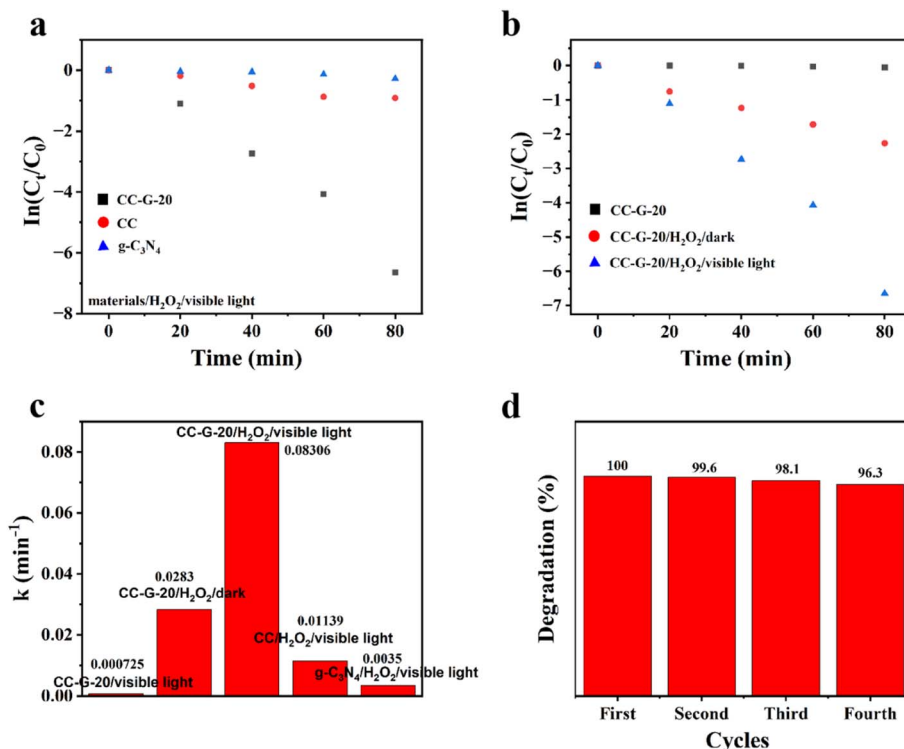
Fig. 7 (a and b) \ln(C_t/C_0) of different catalytic systems (CC-G-20, CC, and g\text{-C}_3\text{N}_4 /visible light/ \text{H}_2\text{O}_2 systems) varied with the reaction time. (c) Reaction rate constants of five catalytic systems in 7(a and b). (d) CC-G-20/visible light/ \text{H}_2\text{O}_2 cycle experiment for MB degradation.
