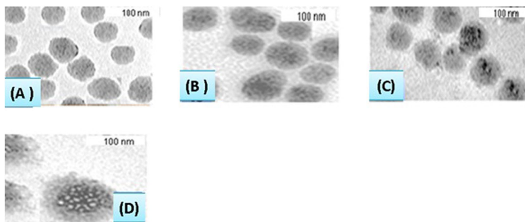
Figure 3. TEM images of DOPE-DOTAP/221 miR sandwiching as an example. (A) DOPE-DOTAP/AuNP. (B) DOPE-DOTAP/AuNP + Stem probe. (C) DOPE-DOTAP/AuNP + Stemprobe + 221 miR. (D) DOPE-DOTAP/AuNP + Stem probe + 221 miR + p19 on the copper grid.
