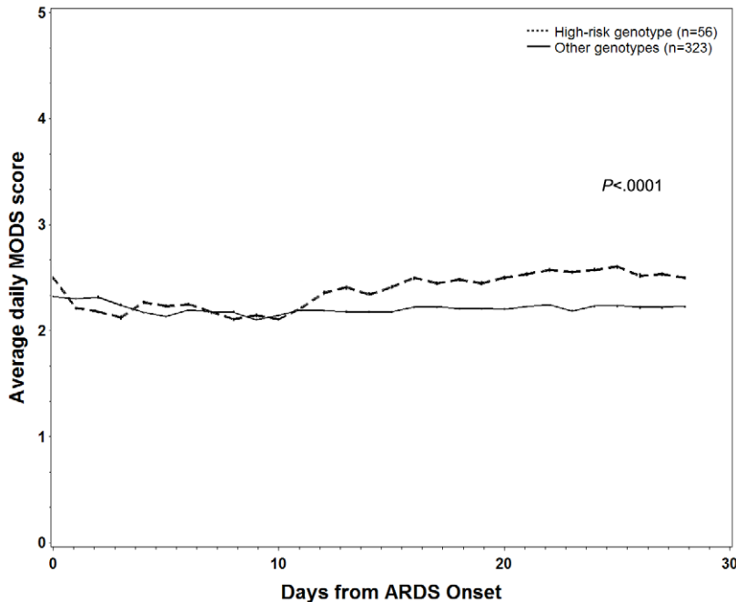
Figure 3. Plot of average daily MODS score by genotype. Graph depicts 28-day MODS for del/del patients vs. all other patients. P-value stated is for mixed effects model adjusting for APACHE III severity of illness score and preexisting organ dysfunction. doi:10.1371/journal.pone.0019469.g003
