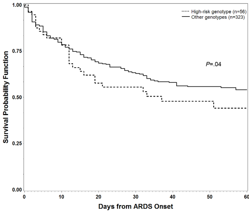
Figure 2. Kaplan-Meier analysis of 60-day survival by genotype. Graph depicts 60-day survival for del/del patients vs. all other patients. P-value stated is for Cox proportional hazards model of adjusted hazard of death within 60 days. doi:10.1371/journal.pone.0019469.g002
