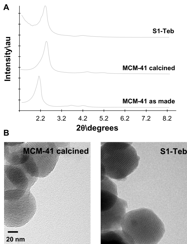
Figure 2 S1-Teb characterization results. (A) Powder X-ray pattern of MCM-41 as made, MCM-41 calcined, and S1-Teb. (B) Transmission electron microscopy image of MCM-41 calcined and S1-Teb. Abbreviations: MCM-41, mobil composition of matter-41; S1-Teb, MCM-41 loaded with tebuconazole.
