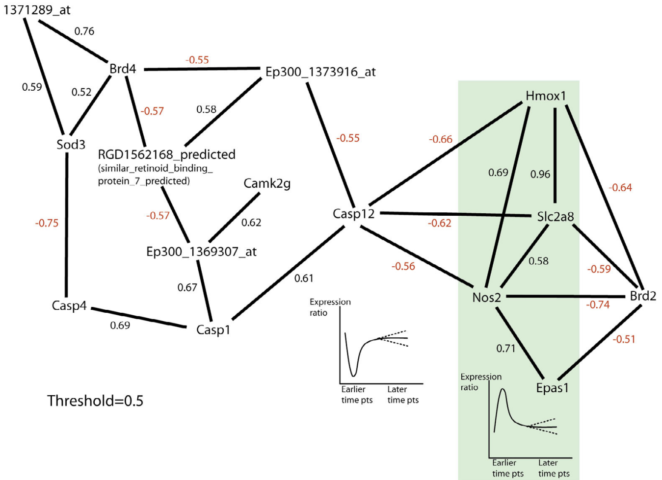
Figure 3 Co-expression network. NOS2, Hmx1, slc2a8, and Epas1 all show a rise in the early time points while Casp12 (and genes positively correlated with it) show an early drop. The figures underneath these genes show this time trajectory with dashed lines showing that the later time points do not necessarily show a flat response. The correlations between genes are shown next to the lines connecting genes.
