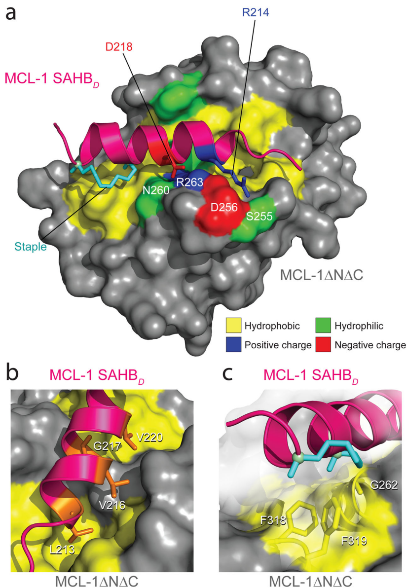
Figure 3. Crystal structure of the MCL-1 SAHB D /MCL-1 N C complex. (a) MCL-1 SAHB D engages MCL-1 N C at the canonical BH3 binding groove of anti-apoptotic proteins, as determined by x-ray crystallography at 2.32-Å resolution (PDB 3MK8). Hydrophobic interactions at the binding interface are reinforced by a complementary polar interaction network that involves MCL-1 SAHB D residues R214 and D218 and MCL-1 N C residues S255, D256, N260, and R263. The side chains of hydrophobic, positively charged, negatively charged and hydrophilic residues are colored yellow, blue, red and green, respectively. (b) The core BH3 residues L213, V216, G217 and V220 of MCL-1 SAHB D make direct contact with a hydrophobic cleft at the surface of MCL-1 N C. (c) The hydrocarbon staple, bearing an olefin in the cis conformation, contributes additional hydrophobic contacts at the perimeter of the core interaction site.
