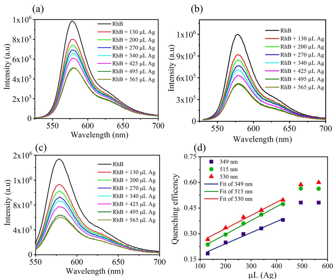
Fig. 6 Fluorescence spectra of RhB (1.2 \mu\text{M} ) in comparison with the mixtures of Ag nanodisks + RhB (1.2 \mu\text{M} ), with the amount of stock Ag nanodisks varying from 130 \mu\text{L} to 565 \mu\text{L} in a titration volume of 1700 \mu\text{L} , under different excitation wavelengths at 349 nm (a), 515 nm (b), and 530 nm (c); (d) fluorescence quenching efficiency of mixed solutions of Ag nanodisks + RhB depending on the amount of stock Ag nanodisks solution and the excitation wavelength.
