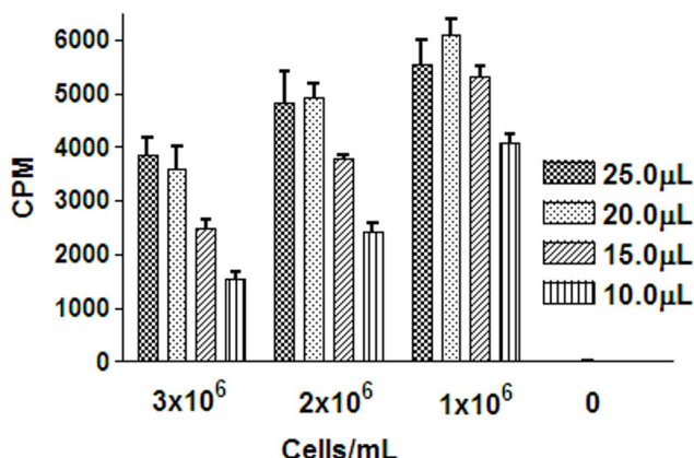
Figure 2 Combination of cell concentrations of T.b.brucei and reagent volumes for signal detection when a 384-well plate inoculated directly from flask culture dilutions and detected by the luciferase ATP detection assay. Fifty-five μL of T.b.brucei cell densities ranging from 1-3 × 10 6 cells/mL were transferred from a flask culture in to a 384 well plate and detected with CellTiter-Glo. Twenty-five, 20, 15 and 10 μL volumes of CellTiter-Glo were compared for signal detection and reproducibility.
