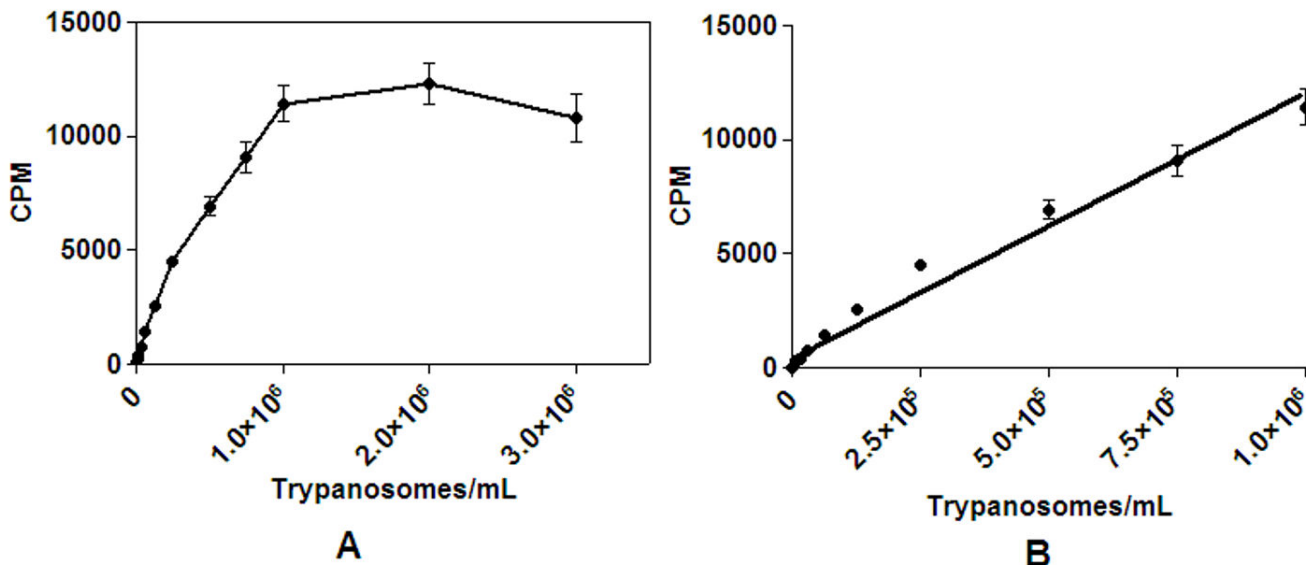
Figure 3 T.b.brucei cells directly transferred from a flask culture to a 384 well plate and ATP detected with 15 μL luciferase based reagent. (A) Cell concentrations of T.b.brucei and detection by the luciferase based assay of 55 μL per well of over a dose range to 3 × 10 6 cells/mL with cells transferred directly from dilutions made from flask grown cultures. 15 μL of luciferase reagent was added for detection. The mean CPM was estimated over 4 replicates from two separate experiments. (B) There was a linear relationship between cell number and trypanosomes to 1 × 10 6 cells/mL (r 2 = 0.99).
