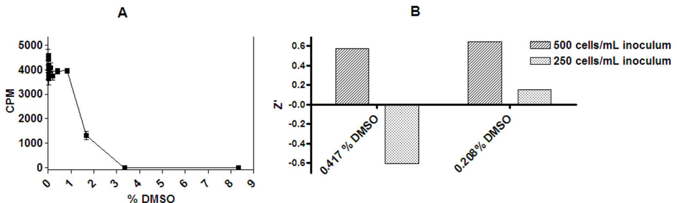
Figure 6 DMSO dose response curve for 500 cells/mL inoculum; and the Z' of pre-diluted DMSO at 0.417% and 0.208% final concentration in the assay for a 500 and 250 cells/mL inoculum density. (A) DMSO standard curve from 0 to 8.3% DMSO in the luciferase assay for a 500 cell/mL inoculum (B) DMSO concentration and Z' of 500 and 250 mL cell inocula with a pre-dilution of DMSO to decrease the assay concentration. The Z' was estimated from a quarter of a 384 well plate.
