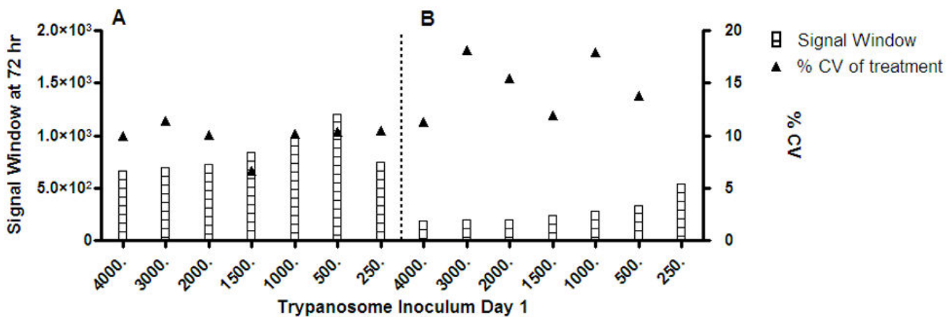
Figure 5 Signal window and % CV of samples from varying inocula of trypanosomes following 72 hours growth and detection with the luciferase viability assay. The assay signal window and % CV after 72 hours growth with differing trypanosome inocula were compared with both 15 \mu L (A) and 10 \mu L (B) of detectant. The signal window was calculated from media without a cell addition.
