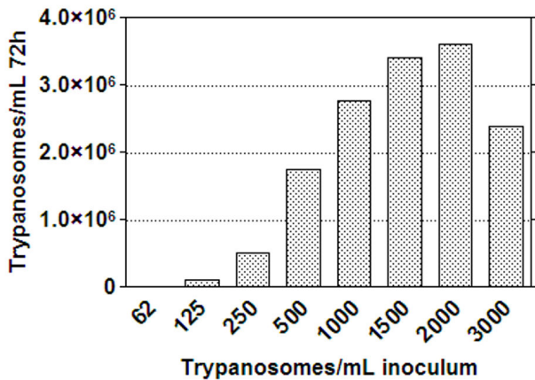
Figure 4 Cell counts of T.b. brucei following growth at 72 hours in a 384-well plate. Varying inocula of trypanosomes were grown in 55 \mu L of HMI-9 media and harvested for counting after 72 hours growth.
