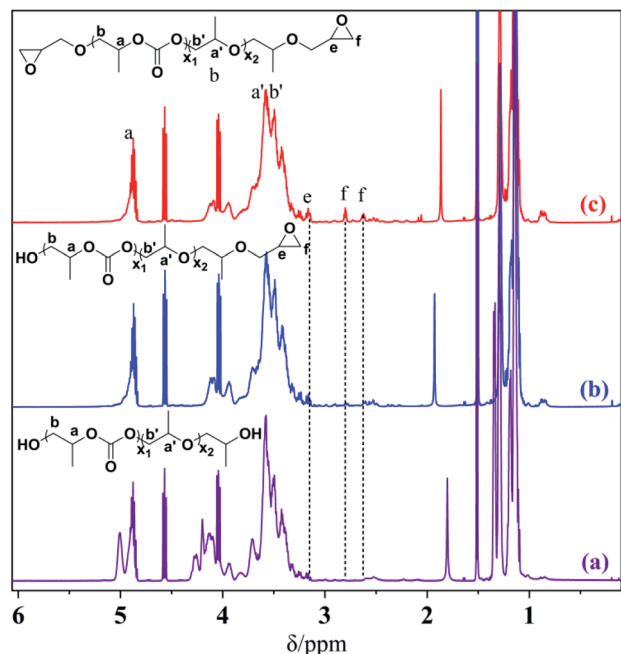
Fig. 1 ^1\text{H} NMR spectra of HO-PPC-OH (a), EP-PPC-OH (b) and EP-PPC-EP (c) (in \text{CDCl}_3\text{-}d , 500 MHz).
