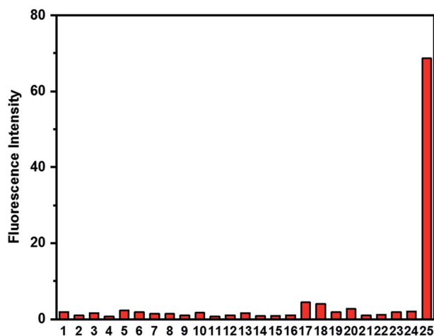
Fig. 4 Fluorescence responses of HCA-OH toward 100 \mu M analytes unless otherwise noted: (1) blank, (2) Na^+ , (3) K^+ , (4) Mg^{2+} , (5) Cu^{2+} , (6) Fe^{2+} , (7) Fe^{3+} , (8) Ca^{2+} , (9) Cl^- , (10) S_2O_3^{2-} , (11) SO_4^{2-} , (12) HSO_3^- , (13) NO_3^- , (14) Cys (5 mM), (15) Hcy (5 mM), (16) GSH (5 mM), (17) \cdot OH , (18) t-BuOOH , (19) ^1O_2 , (20) NO, (21) NO_2^- , (22) H_2O_2 , (23) O_2^{\cdot -} , (24) ClO^- , (25) ONOO^- (30 \mu M). The final concentration of HCA-OH was 10 \mu M. All experiments data were collected in PBS buffer (10 mM, pH 7.4) with 1% DMSO at 37 °C. The excitation and emission wavelengths were 460 nm and 548 nm, respectively.
