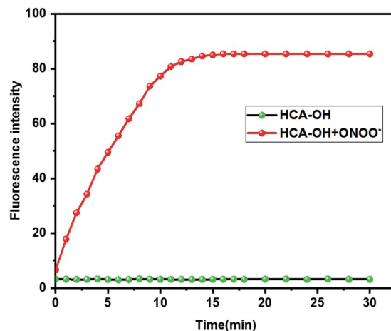
Fig. 2 Time-dependent changes in the fluorescence intensity of HCA-OH (black line: 0 \mu\text{M} ONOO - , red line: 30 \mu\text{M} ONOO - ). The excitation and emission wavelengths were 460 nm and 548 nm, respectively.
